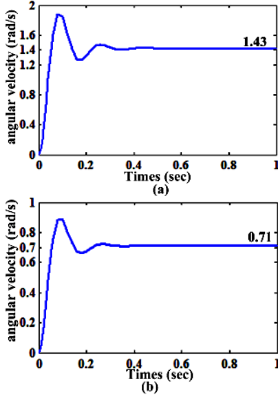
Fig. 5. The results of the simulation with no load: (a) with 10 v as the input signal, (b) with 5 v as the input signal
