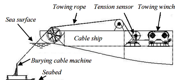
Fig. 1. The towing winch in the sea cable burying system
