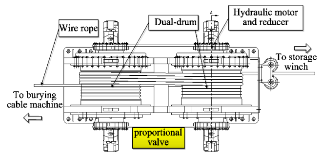
Fig. 2. The towing winch
