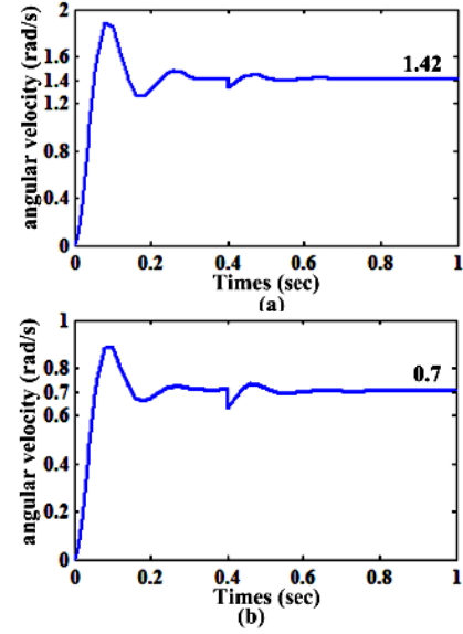
Fig. 7 The results of the simulation with 3 ton load: (a) with 10 v as the input signal, (b) with 5 v as the input signal
