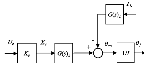
Fig. 3. Transfer function block diagram of the winch hydraulic system
