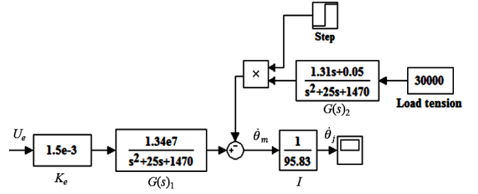
Fig. 6. Block diagram of the winch model with 3 ton load
