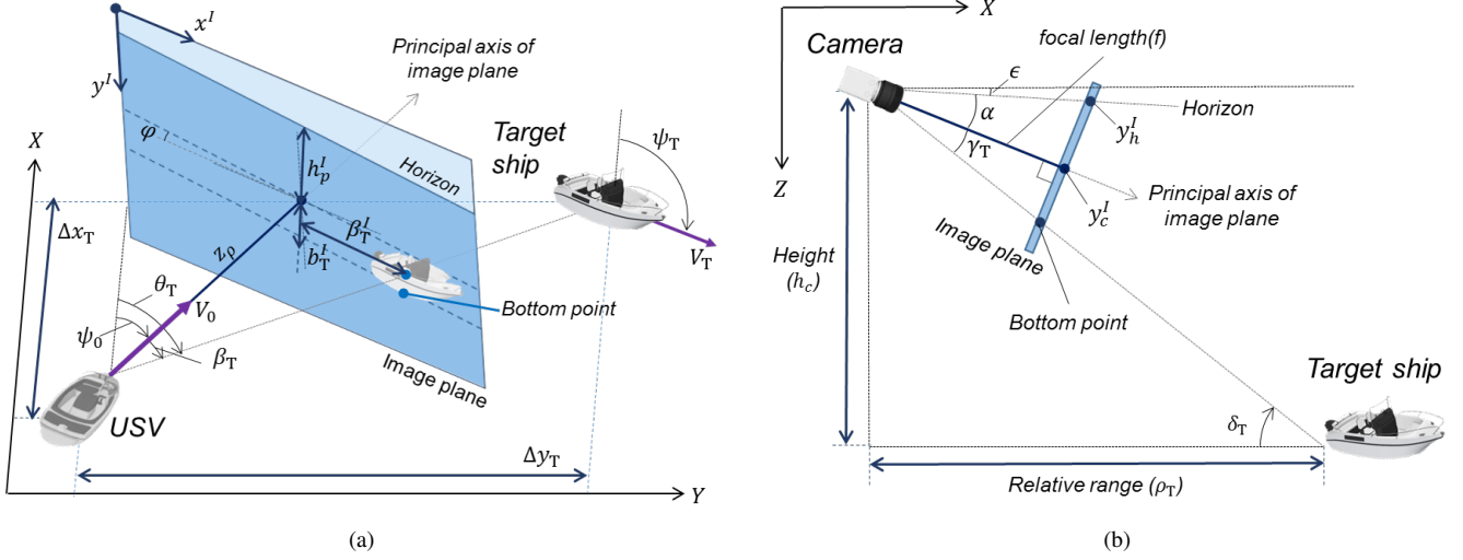
Fig. 3: Camera geometry and coordinate systems: (a) Coordinate systems in the horizontal plane for bearing measurements; (b) Coordinate systems in the vertical plane for range measurements.
