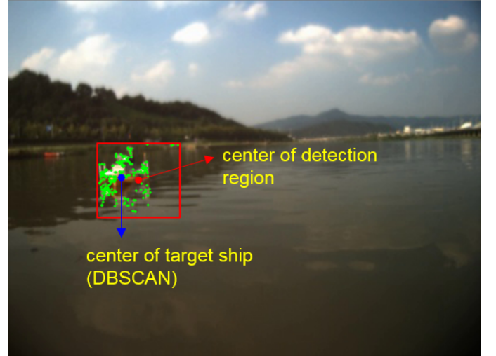
Fig. 4: Results of the center point of the detection region and DBSCAN. The green dots represent feature points extracted by the FAST corner detector in the detection region.
