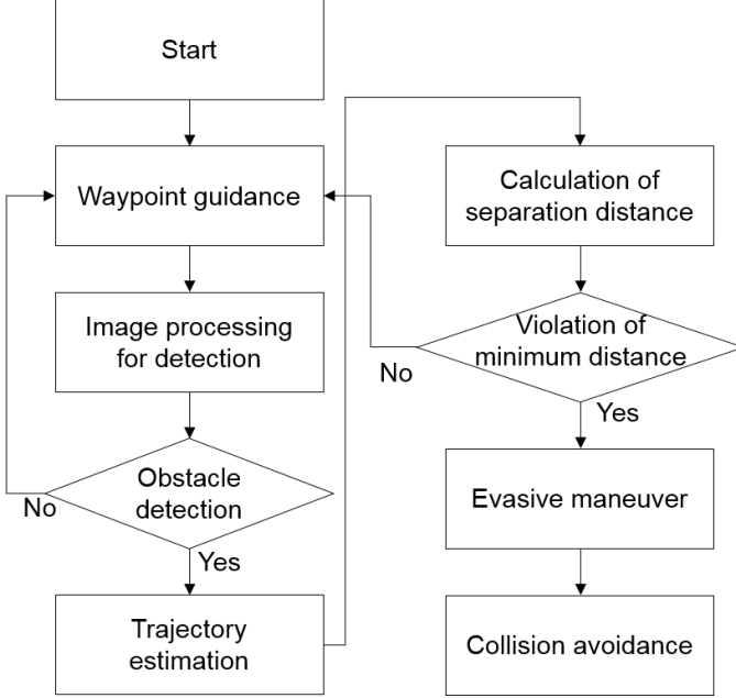
Fig. 1: A procedure of the vision-based collision avoidance for autonomous navigation.
