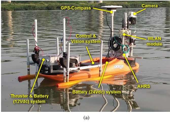
Fig. 5: Two vehicles used in the on-water experiment: (a) Orange duck (Length 2.2 m), the observer; (b) Yellow duck (Length 2.8 m), the target ship
