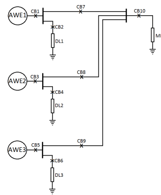
Fig4: Modeled Offshore AWE farm
