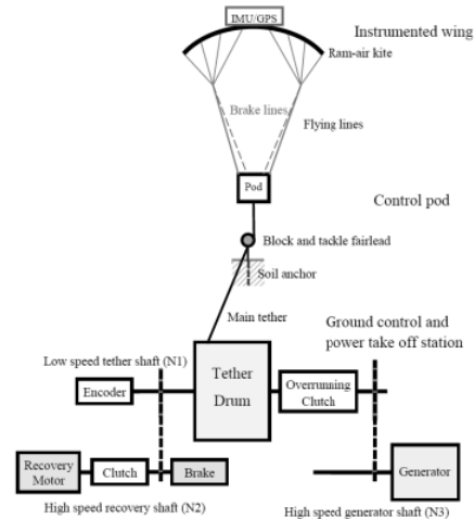
Fig1. Pumping-mode airborne wind energy system, with non-reversing generator [1, 5]
