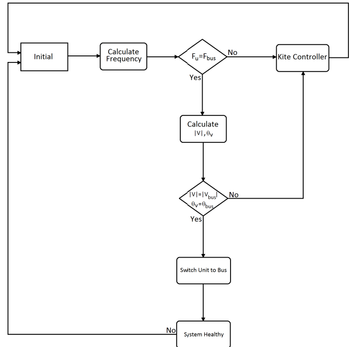
Fig3: Synchronization Algorithm
