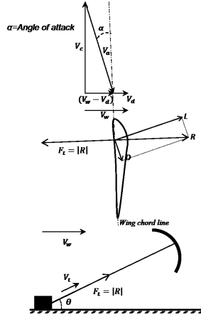
Fig5: Aerodynamic Forces during crosswind flight [1, 5]
