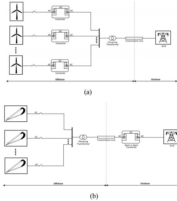
Fig2: Interconnection of offshore devices, (a) Conventional approach, (b) Proposed approach
