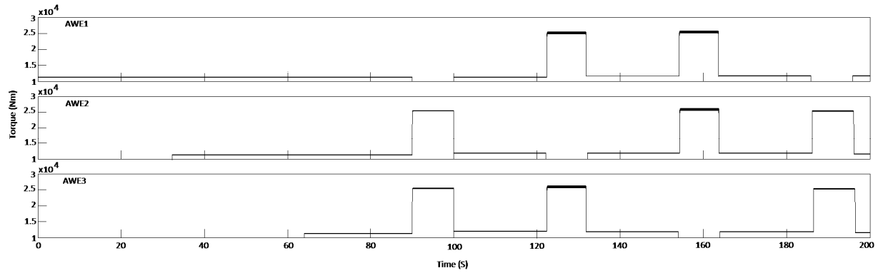
Fig7: Mechanical Torque
