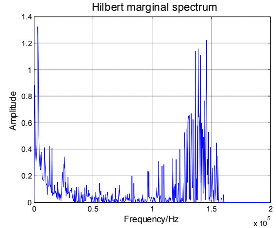
Fig. 6. The Hilbert marginal spectrum of finless porpoise signal
