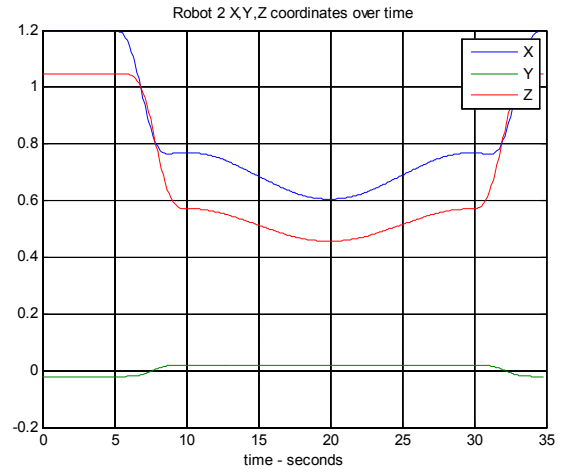
Fig. 8. Cartesian End-effector x, y and z Coordinates over Time for Robot 2 for Scenario 1 Simulation
