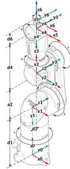
Fig. 5. Kinematics Model of Staubli TX60 Robot
