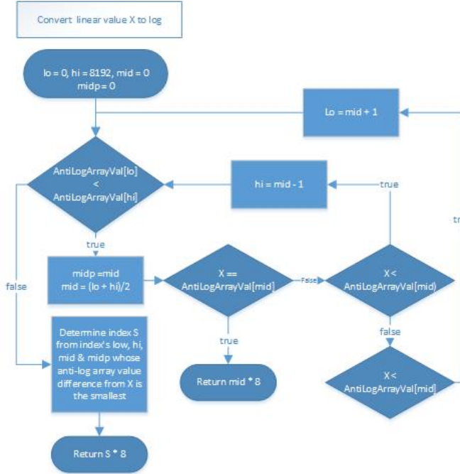
Figure 5 Anti-Log Binary Search
