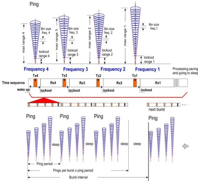
Figure 2 Schematic of the instrument sampling scheme showing the timing for individual pings and bursts.
