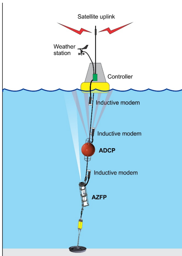
Figure 3 Mooring with Inductive Modems
