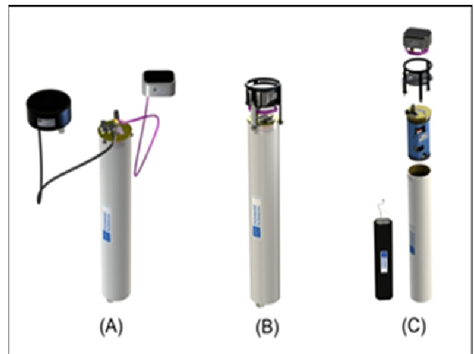
Figure 1 Configuration of the AZFP: (A) with the 38 kHz channel, (B) as a 4-frequency 125/200/455/770 combination, (C) as an exploded view.
