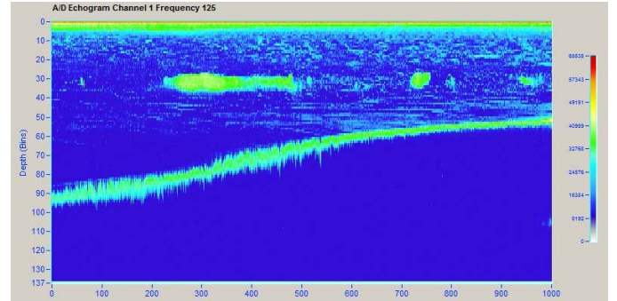
Figure 7 Condensed Profile to 1/50 Resolution
