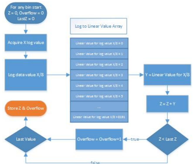
Figure 4 Log to Linear Conversion
