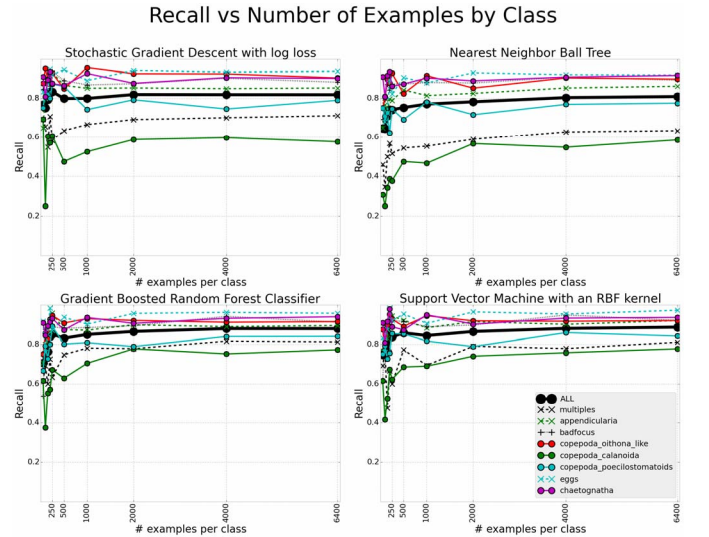
Fig. 7. Difficult classes tended to remain difficult, regardless of algorithm or data set size.
