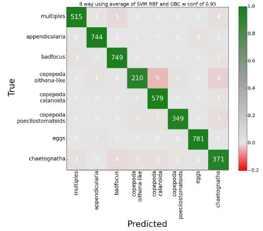
Fig. 11. Confusion matrix when the classifier is allowed to abstain from labeling images and only classifying when probability exceeds 0.95. This approach greatly reduces the number of false positives compared to other classifiers.
