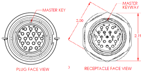
Figure 5. Plug and Receptacle Face Patterns: 19 way Base
