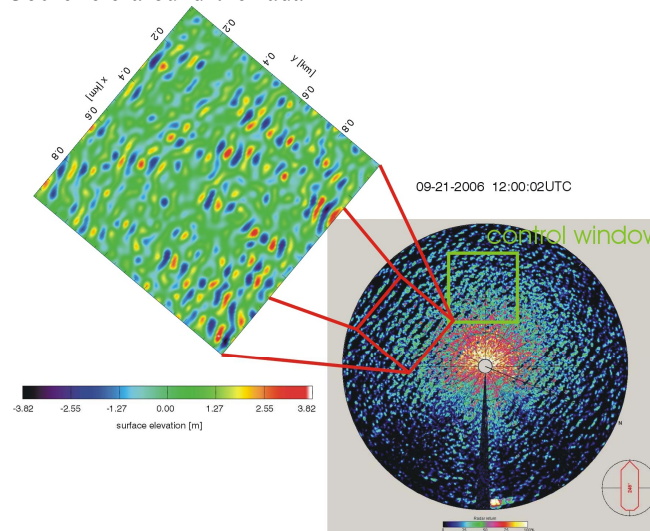
Figure 3: The window positioning algorithms focuses the wave analysis to areas with approaching waves.
