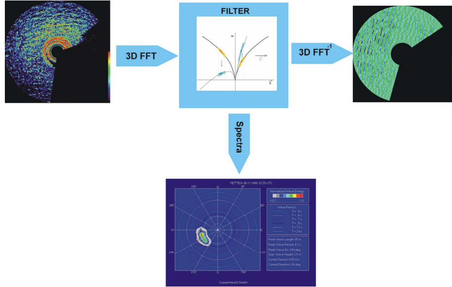
Figure 2: Deriving the sea surface elevation from radar images.
