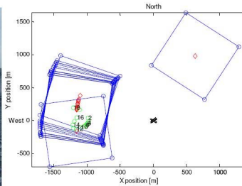
Figure 4: Drifting wave rider buoy and radar analysis window are shifted to the same positions. The exact positions of both sensors and the timing is very relevant to carry out any data comparisons.
