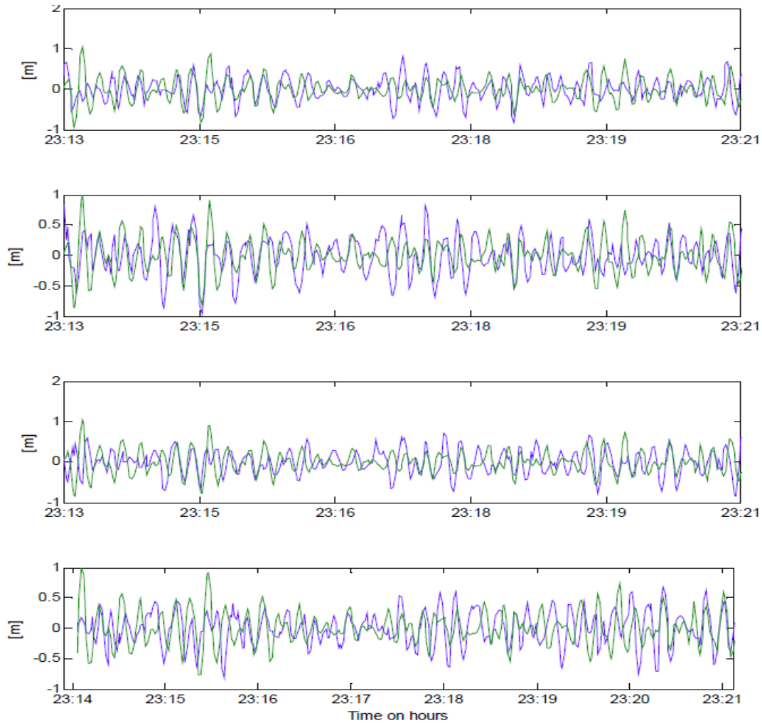
Figure 6: Vessel heave motion predicted 42, 60, 90 and 120 seconds in advance by OWME system compared with the measured on board heave motion (trials on an Offshore Support Vessel at Gulfaks field, September 2008). The green lines represent the measured heave motions, the blue lines the predicted motions.
