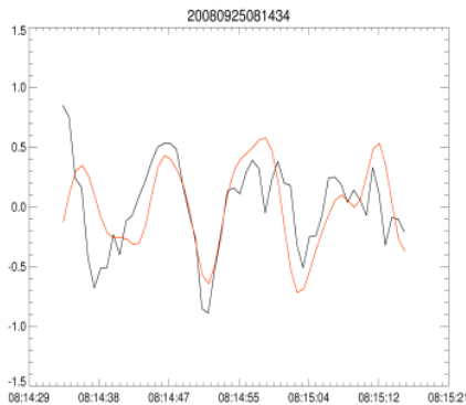
Figure 5: Comparison between wave elevation derived from WaMoS (red) and buoy (black).
