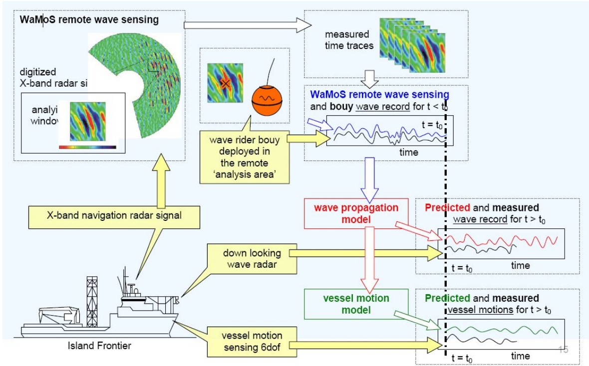
Figure 1: OWME real time prediction scheme. Sea surface elevations are retrieved from X-band radar data. A 1-D wave height series is then fed into a wave forecasting model, which then is used as input to the vessel motion prediction model.
