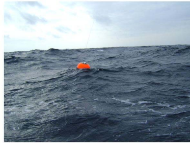
Figure 4: Drifting wave rider buoy and radar analysis window are shifted to the same positions. The exact positions of both sensors and the timing is very relevant to carry out any data comparisons.
