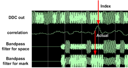
Figure 16. Snapshot of hardware simulation result for 12'' bucket test
