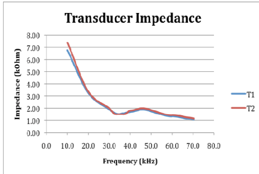
Figure 4. The transducer impedance and resonance frequency ( \sim 35kHz) of transducers potted from ceramics T1 and T2
