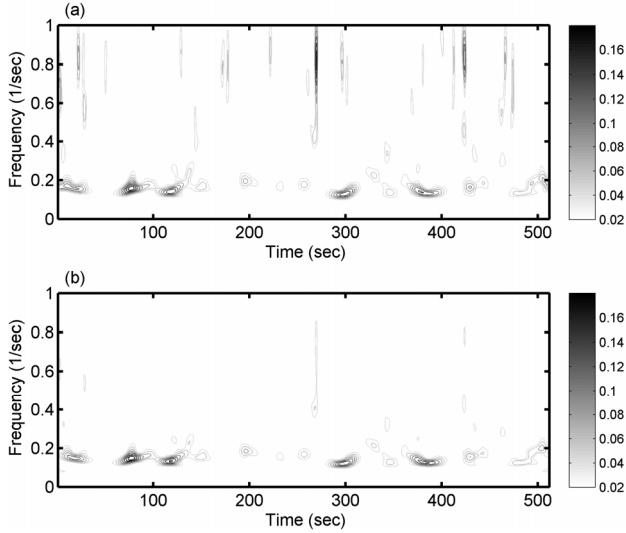
Figure 3. Wave scalograms calculated from the sea surface elevation signals (a) and wave acceleration signals (b).
