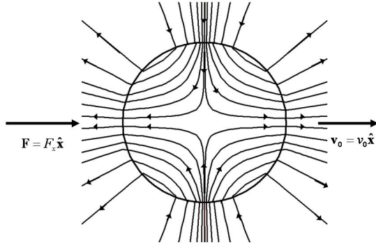
Fig.3. Lines of anomalous magnetic field within and around a spherical cavity due to the water flow component parallel to the geomagnetic field. The view is a section containing \mathbf{v}_0 and \mathbf{F} , through the centre of the sphere. The field is rotationally symmetric about the x axis. Inside the cavity the gradient is uniform, with maximum gradient parallel to the x axis.
