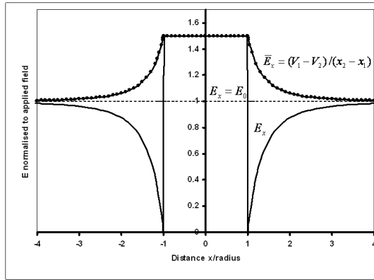
Fig.1. Normalized electric field (E) profile, parallel to the uniform applied field, passing through the centre of a spherical cavity. Solid line indicates the local field; the horizontal dashed line represents the unperturbed applied field; the line with dots shows the average field over a baseline defined by symmetrically placed potential electrodes.
