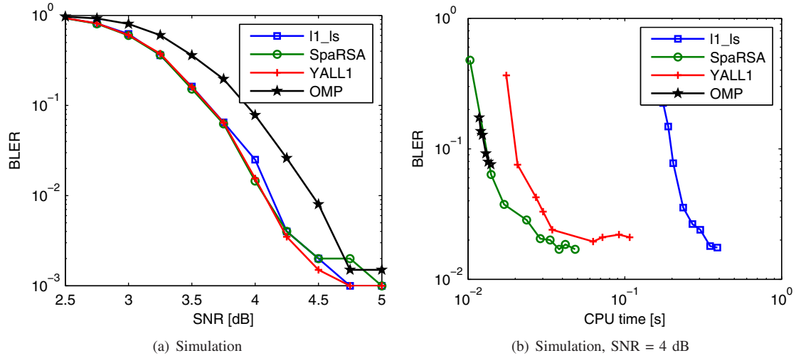
Fig. 3. MIMO with ICI-ignorant receivers, N_t = 2 , N_r = 4 , 16QAM, 1000 runs.
