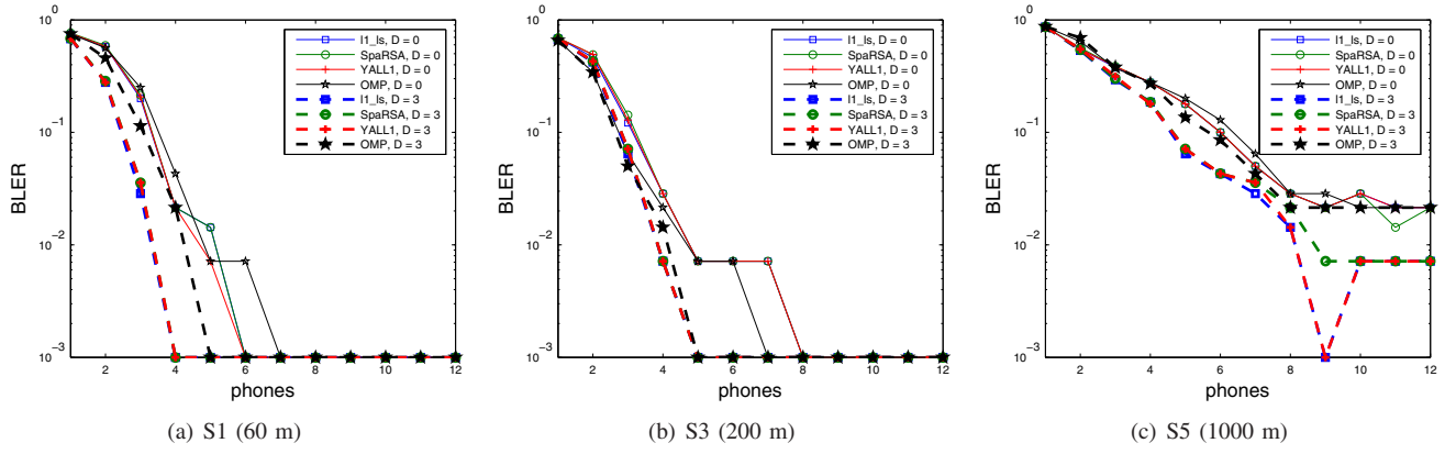
Fig. 2. SIMO with ICI-ignorant and ICI-aware receiver, 16-QAM, Julian date 300, SPACE08.
