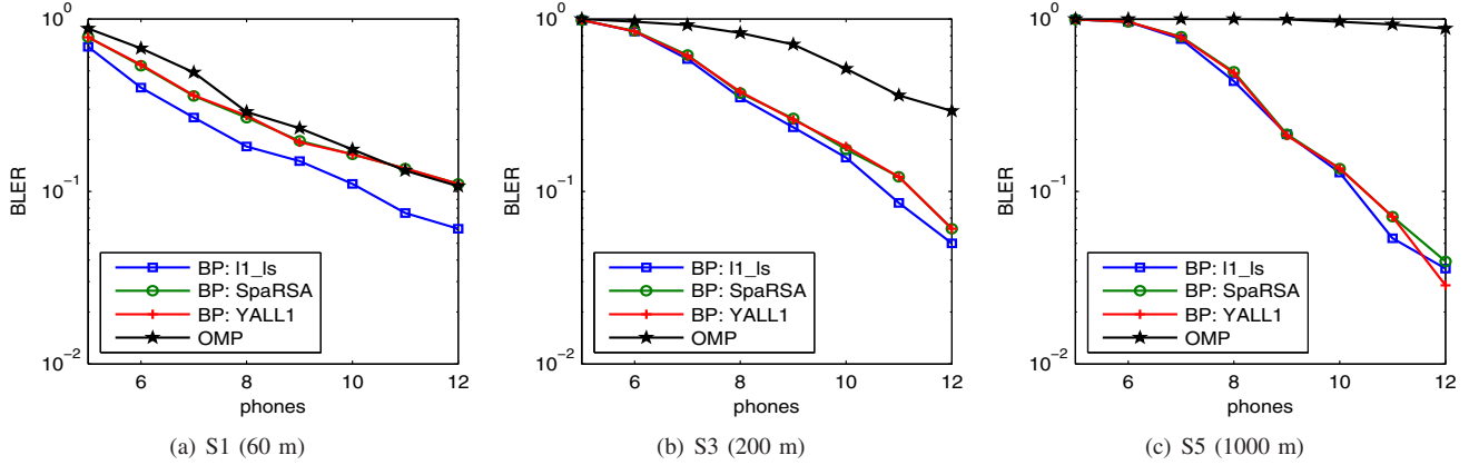
Fig. 4. MIMO with ICI-ignorant receivers, SPACE08, Julian date 298.
