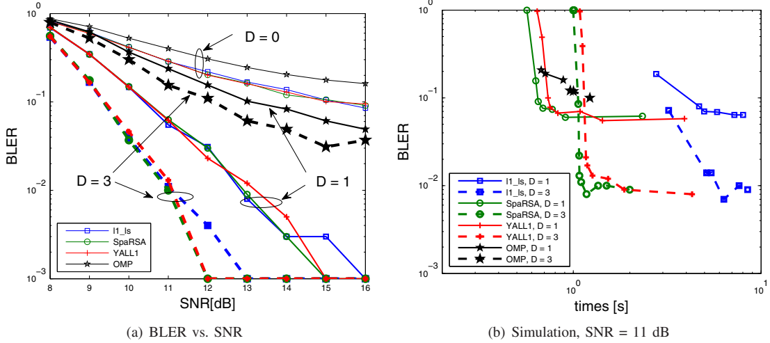
Fig. 1. SIMO with ICI-aware and ICI-ignorant receivers, 16 QAM. The overview of CPU time is shown in Table I.
