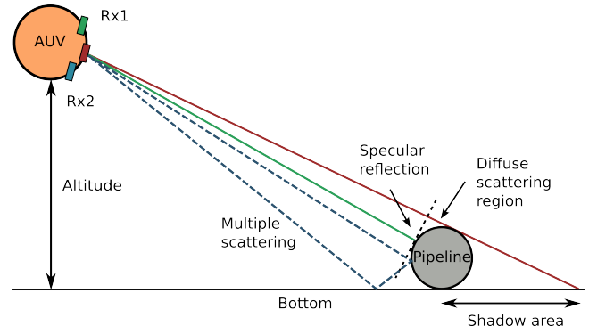
Fig. 9. Scattering geometry
