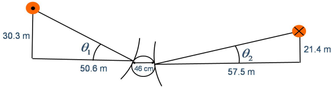
Fig. 14. Geometry of a two-sided pipeline survey. The orange circle at the upper left section is the AUV travelling out of the paper and the one at the upper right illustrates the AUV traveling into the paper. The measured width between the specular reflections, w , is equal to 46 cm.
