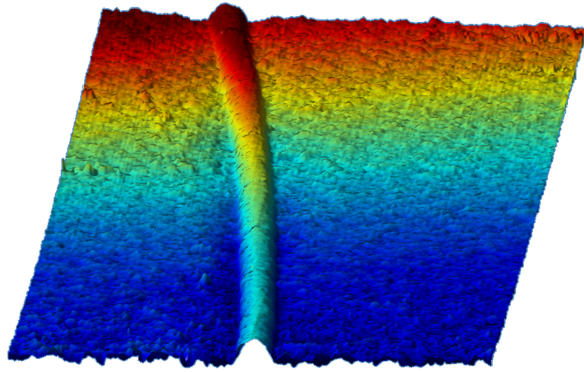
Fig. 17. A 8 by 100 meter zoom of a 100 meter section of the pipeline bathymetry in Figure 16. Note that the aspect ratio is not equal in the horizontal plane. The relative height of the pipeline is approximately 30 cm.
