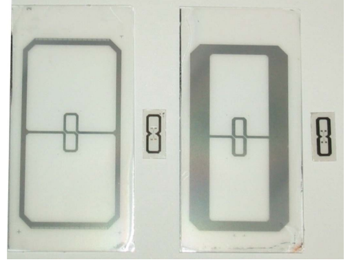
Figure 3. Picture of the two device designs A and B, with the larger gradiometric flux transformers on the left and the smaller readout gradiometers on the right.
