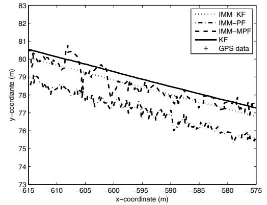
Fig. 2. Trajectory tracking result in detail.
