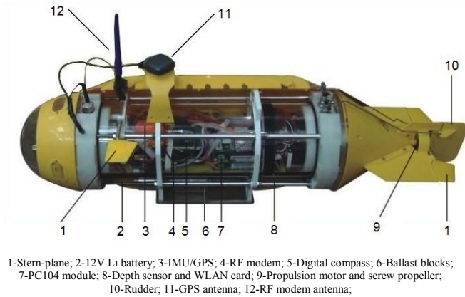
Fig.2 A picture of the AUV
