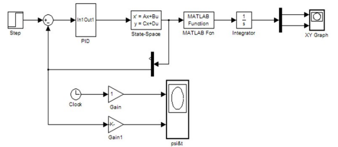
Fig.4 AUV's linearized simulation model
