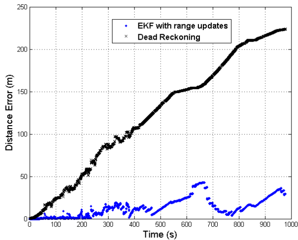
Fig. 11. Position error of EKF with range updates (cooperative positioning) as compared with dead reckoning (single AUV positioning) during sea trials
