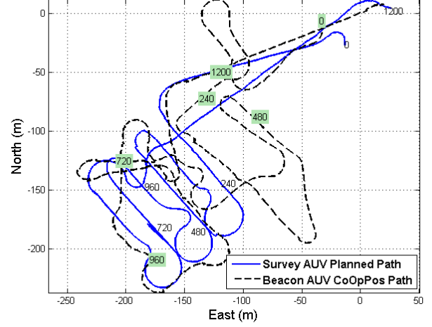
Fig. 5. AUV paths for lawnmower mission survey during lake trial
