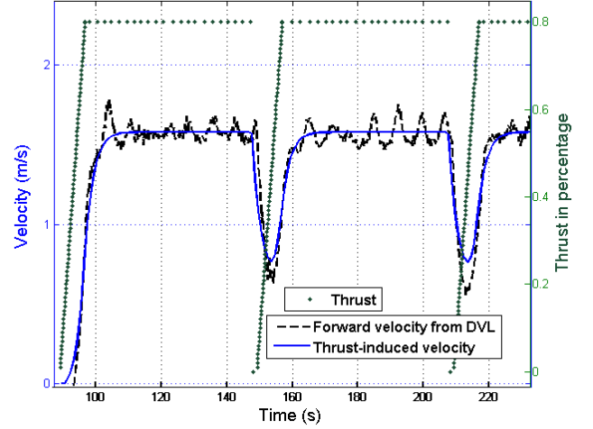
Fig. 2. Thruster model estimating forward velocity of AUV compared with the velocity measurement from DVL. The dotted line shows the thruster control signal.
