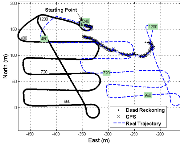
Fig. 8. Survey AUV: drift due to ocean currents during sea trials (single AUV positioning)
