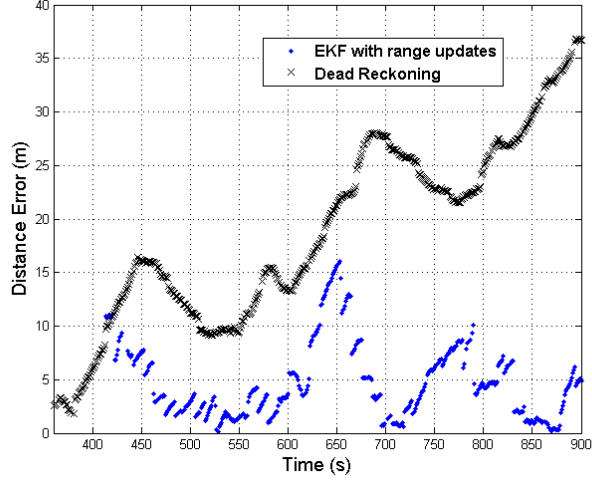
Fig. 7. Position error of EKF with range updates (cooperative positioning) as compared with dead reckoning (single AUV positioning) during lake trials
