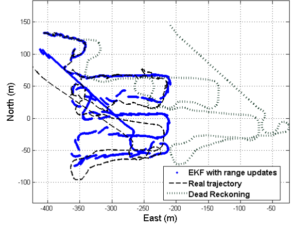
Fig. 10. Comparison EKF with ranging (cooperative positioning) and dead-reckoning (single AUV positioning) during sea trials
