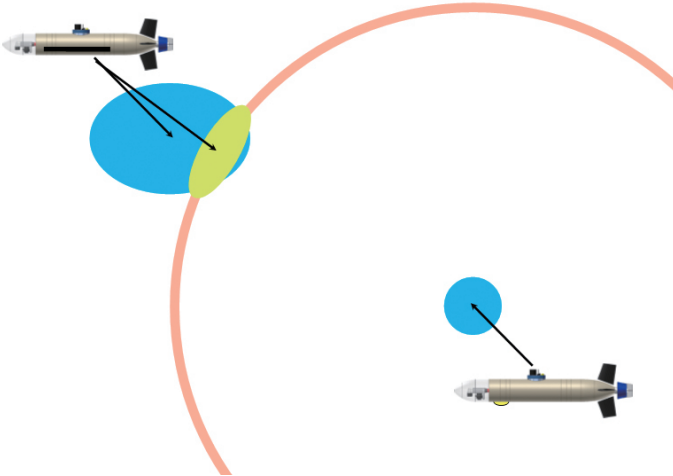
Fig. 4. Illustration of error estimates by range measurements
