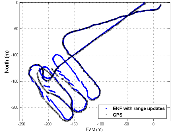
Fig. 6. Survey AUV: EKF with range updates (cooperative positioning) compared with GPS data during lake trials
