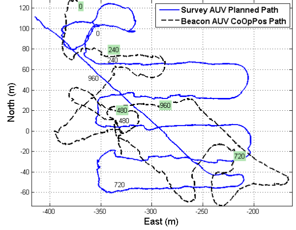
Fig. 9. AUV paths for lawnmower mission survey during sea trials
