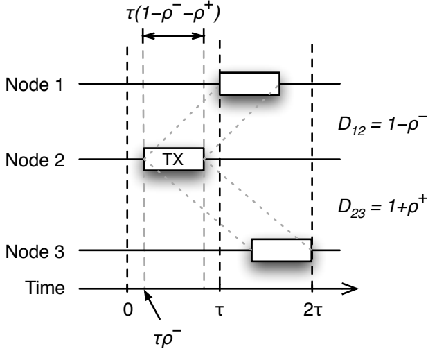
Fig. 2. An illustration of a \rho -schedule
