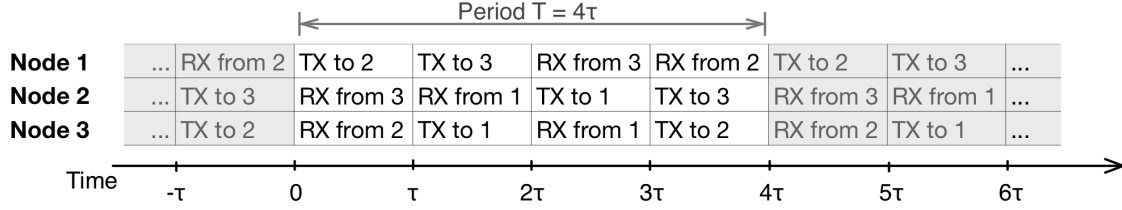
(b) Periodic schedule
