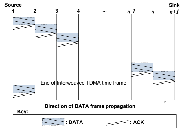
Fig. 2. Timing diagram for strictly hop-by-hop Stop & Wait ARQ on Interweaved TDMA MAC.
