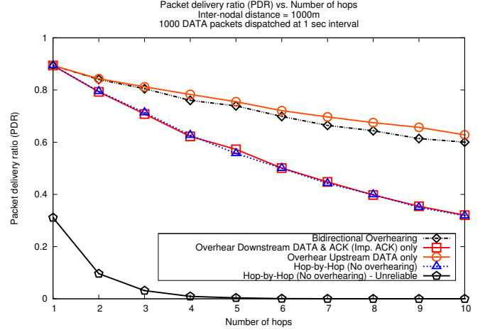
Fig. 8. Simulation results of packet delivery ratio (PDR) plotted against the number of hops. A maximum retransmission of 5 was used by all schemes except Hop-by-Hop - Unreliable, which transmits each DATA frame a maximum of 1 time. This reflects both the adverse conditions of the channel model and the beneficial effects of retransmissions.
