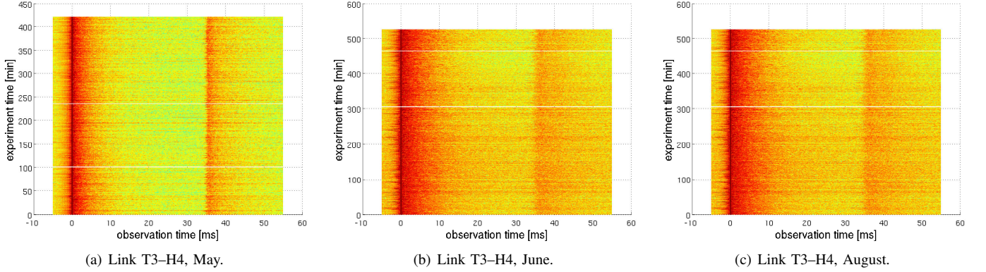
Figure 4. Pseudocolor plot of measured channel impulse response amplitudes for the link between T3 and H4.
