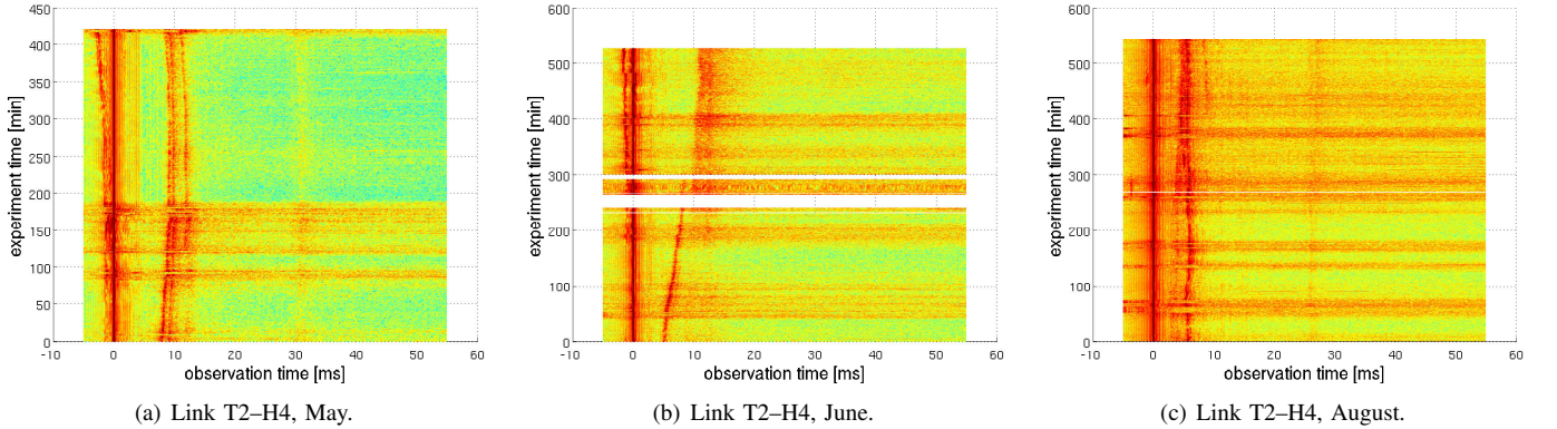
Figure 5. Pseudocolor plot of measured channel impulse response amplitudes for the link between T2 and H4.
