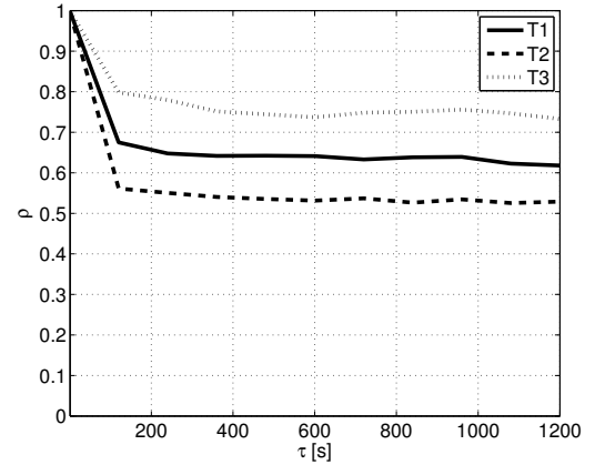
Figure 15. Channel correlation coefficient \rho as a function of time lapse \tau in June predicted by Bellhop. The links considered are from each transmitter T1, T2, T3 to hydrophone H4.
