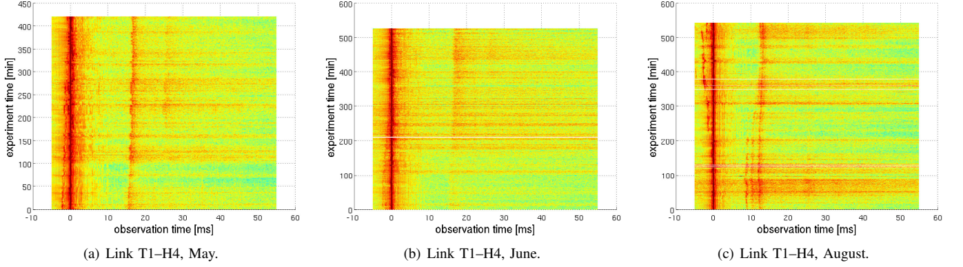
Figure 3. Pseudocolor plot of measured channel impulse response amplitudes for the link between T1 and H4.
