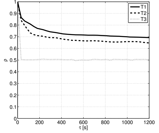
Figure 8. Channel correlation coefficient \rho as a function of time lapse \tau in August. The links considered are from each transmitter T1, T2, T3 to hydrophone H4.
