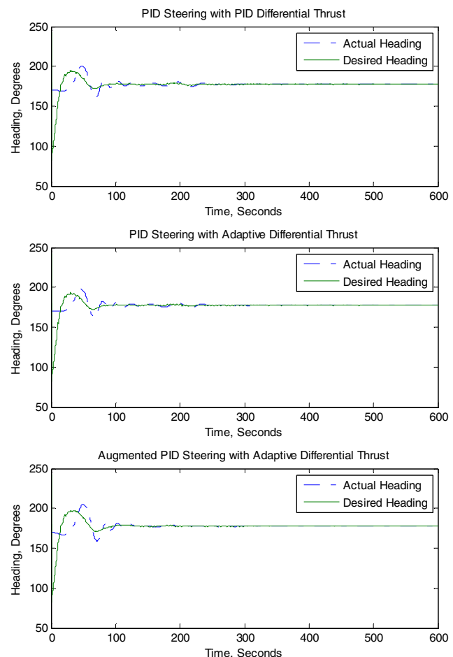
Figure 2: Plot of Actual and Desired Heading, 2 m/s West Wind
