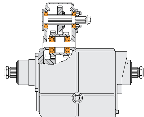
Oil-Splash Lubrication
