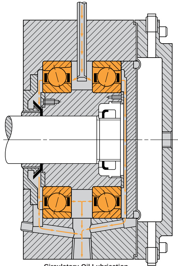
Circulatory-Oil Lubrication
