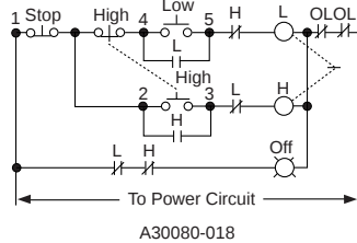
One pilot light "OFF"
