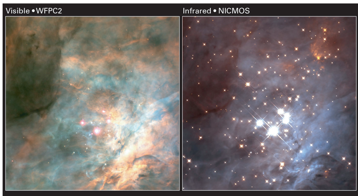
FIGURE 3.11 An illustration of the power of near-infrared light to penetrate dust clouds and reveal embedded, newly formed stars. (left) A Wide-field Planetary Camera 2 (WFPC2) view of the center of the Orion nebula with the five Trapezium stars. (right) The same region imaged in the near infrared with the NICMOS camera, which makes many previously hidden stars visible. This pair of images illustrates why observing at many different wavelengths is required. Wide-field Camera 3 will be 50 times more efficient than NICMOS for this work. Courtesy of STScI/NASA.
