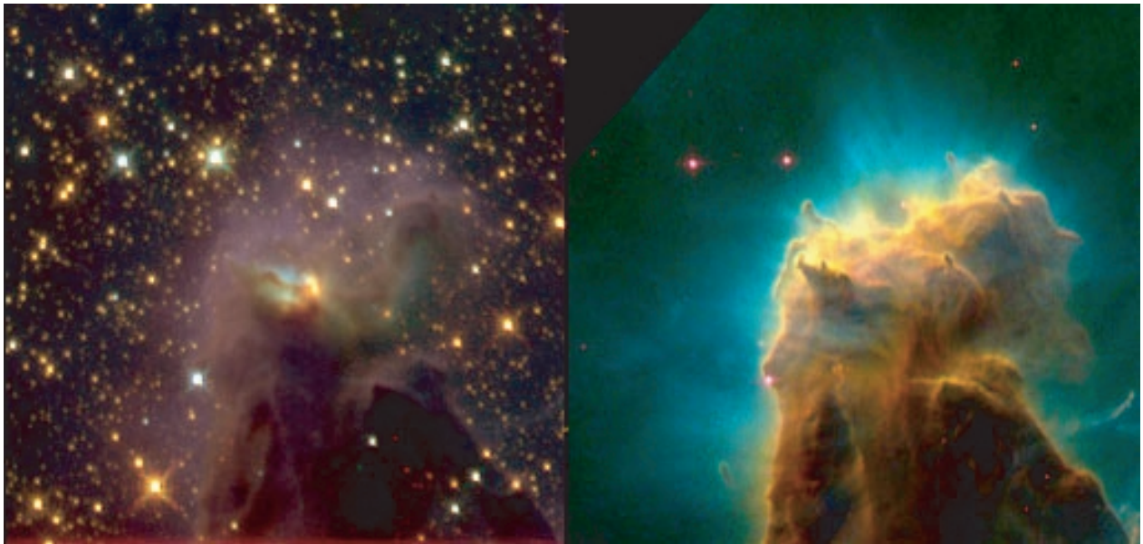
FIGURE 3.2 Two Hubble Space Telescope images illustrate the value of observing at different wavelengths. (left) An image obtained at near-infrared wavelengths, which penetrate the dust, reveals hundreds of stars in the region, as well as a large complex of newly forming stars deep within the dusty column itself. (right) An image obtained at visible wavelengths shows a column of obscuring dust and gas in the famous Eagle nebula (M16). The sculpting away of the dust by an intense rain of radiation from nearby hot stars (off image to top) reveals denser globules of gas inside the column that are seen as protuberances on the surface of the cloud. These protuberances are likely sites of star formation.
