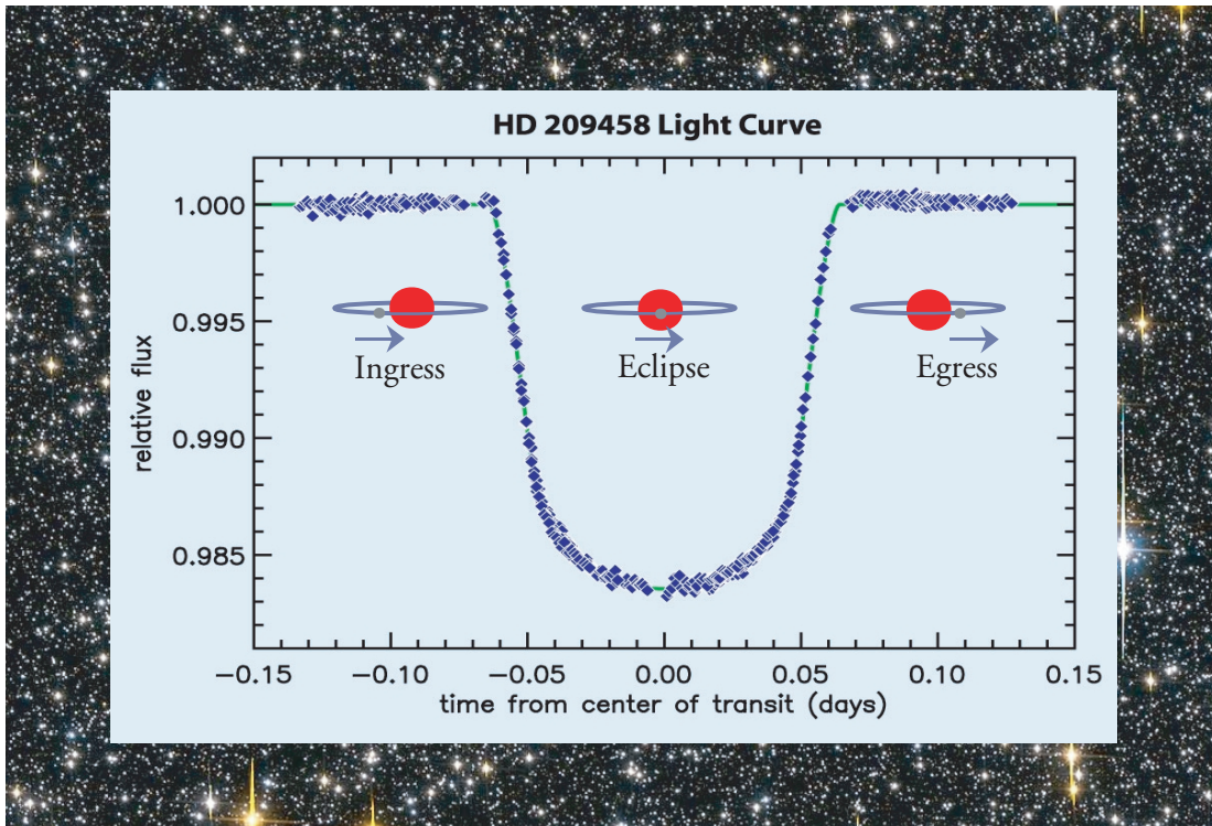
FIGURE 3.10 The presence of an otherwise invisible planet can be detected by the small drop in light caused as the planet travels in front of its parent star. The “light curve” of such a transit is shown here, with the drop in light at slightly more than 1.5 percent, as would occur with a giant Jupiter-like planet passing in front of the Sun. However, the scatter in the Hubble measurements is so small that even smaller planets could be detected. Hubble has begun to monitor rich star fields like that shown in the background, which is a region near the center of the Milky Way Galaxy. In this manner, several hundred thousand stars can be searched for Jupiter-size and smaller planets in roughly 1 week of Hubble Space Telescope observing time. Courtesy of STScI/NASA.
