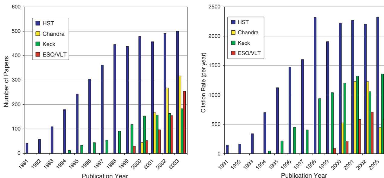
FIGURE 3.5 (left) The number of refereed scientific papers produced annually based on work enabled by major leading telescopes. (right) The number of citations in the scientific literature annually to papers produced from work enabled by major leading telescopes. The criteria used to assign papers to a telescope are parallel for all the telescopes shown here.
