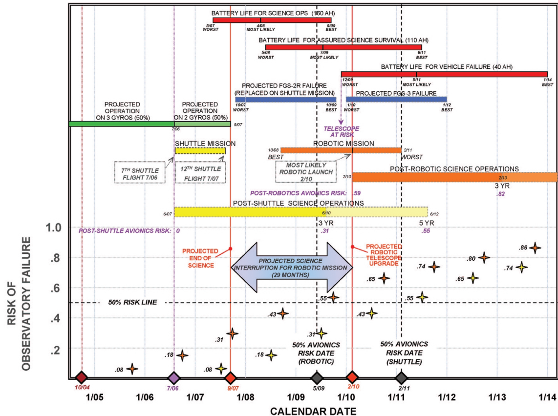
FIGURE 4.3 Hubble Space Telescope system lifetime and servicing assessment, a composite summary of key factors that affect the operational status of HST and the timing for servicing. The upper six red, blue, and green segments are identical to those shown in Figure 4.2 and represent, respectively, the projected lifetime of the batteries, the degraded fine-guidance sensor (FGS) units, and the gyroscopes, based on current patterns of usage. The yellow and orange segments represent the potential servicing windows for a shuttle mission and a robotic mission based on analyses in subsequent chapters and the resulting time line for a 3- to 5-year post-servicing period of science operations. The timing for a shuttle servicing mission is based on a realistic estimate of the dates for the 7th and 12th missions after return to flight, assuming a return to flight in mid-2005. The timing for a robotic mission is based on the 5.4-year “most likely” development period using historical data for NASA missions and the very high level of mission complexity. To represent the potential range of mission dates, a 4-year best case (high risk) and 6.4-year worst case (low risk) are also shown, even though these extreme values are considered unlikely. The blue arrow indicates the projected interruption in the flow of data for science that would result from combining the projected end of science operations based on gyro failure and the most likely date for a robotic mission. The bottom section of the diagram also represents the risk of HST’s failure based on the timing and the method of servicing. (Risk rather than reliability is used in this case in order to be consistent with subsequent chapters and can be derived from the reliability values discussed in the section titled “Avionics Reliability Model” by subtracting the reliability numbers from 1.00). The risk values indicated by orange stars represent the risk to HST of a robotic mission beginning at time zero in October 2004 and progressing forward. The 50 percent risk point for the robotic mission value (orange stars) occurs in May 2009, slightly after the projected servicing window opens, but before the most likely robotic service date. The associated post-robotic science operations are seen to begin with a risk factor (0.59) already above the typical NASA limit of 50 percent,
