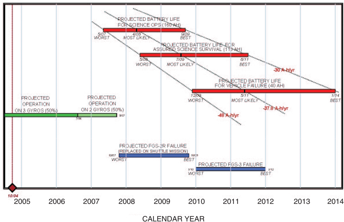
FIGURE 4.2 Lifetime projection for key Hubble Space Telescope subsystems subject to wear-out. The red segments represent the range of projections for HST battery life for capacity levels corresponding to operational state transitions: 160 Ah represents the limiting capacity for supporting science operations, and 40 Ah represents the limiting capacity for protecting the telescope optics from permanent failure. The three dotted lines correspond to the range of expected loss of battery capacity, -37.8 Ah per year being the most likely rate of degradation. The bounding trend lines for worst and best performance are -48 Ah per year and -30 Ah per year, respectively. The green segment shows the projected time for operation of the remaining four working gyroscopes on HST, with the dark green segment representing projected operation of three gyros before failures (of two of the remaining four units) force a transition to a two-gyro operational mode. The light green segment represents the time duration for operating on two gyros before the failure of one more unit results in the suspension of science operations. The blue segments represent the worst- and best-case estimates for the point of failure of the fine-guidance sensors FGS-2R and FGS-3, based on current trends. FGS-2R is projected to fail due to radiation damage sometime between October 2007 and October 2009. Failure of FGS-3 is projected to occur sometime between January 2010 and January 2012, although it should be possible to extend its life if FGS-1R and FGS-2R are used instead when possible.
