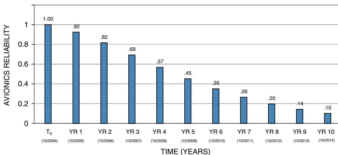
FIGURE 4.1 Hubble Space Telescope avionics system reliability over time. The values shown are as of October 2004, at which time the avionics were working and also retained full redundancy. System failure in the context of this figure means that a combination of component failures have occurred (typically failure of both a prime and a redundant subsystem) such that the HST avionics system is no longer capable of supporting science operations. Due to the nature of the system model, as long as the system continues to operate without failure, the same curves translate forward in time with a starting value of 1.0. The risk values associated with these numbers are calculated as 1 minus the values plotted.
