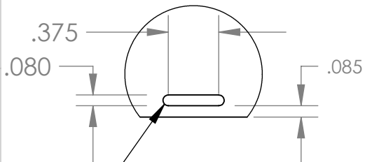
DETAIL D SCALE 1 : 1
