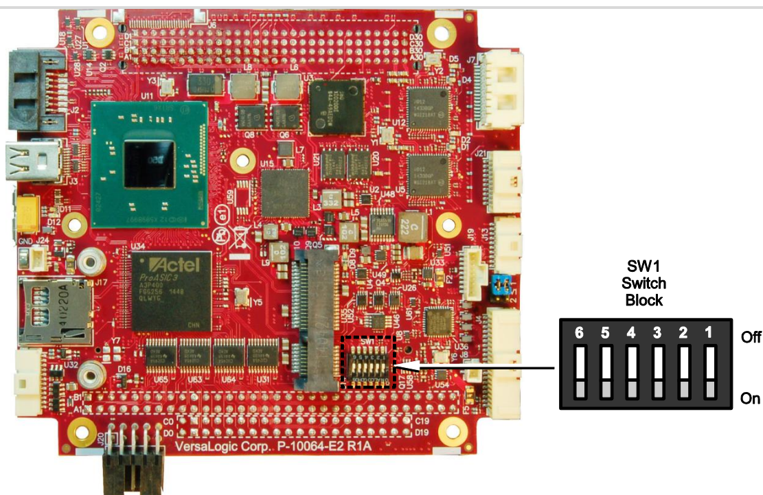
Figure 7. Location of SW1 Configuration Switch Block
