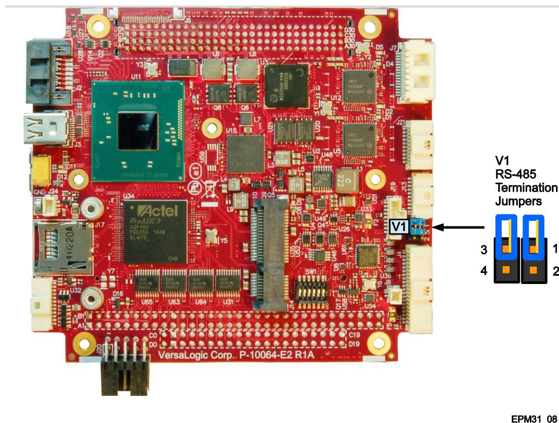
Figure 21. COM1/COM2 End-point Termination Jumpers
