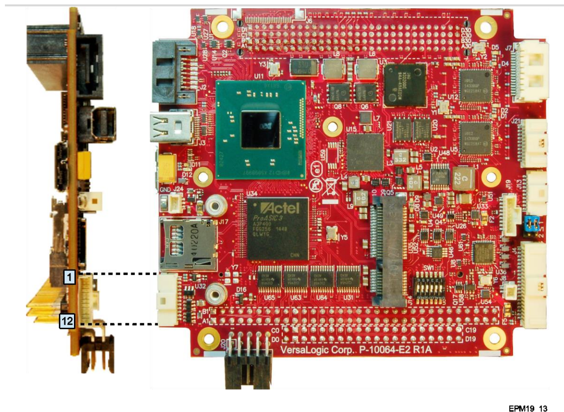
Figure 22. VGA Connector Location and Pin Configuration
