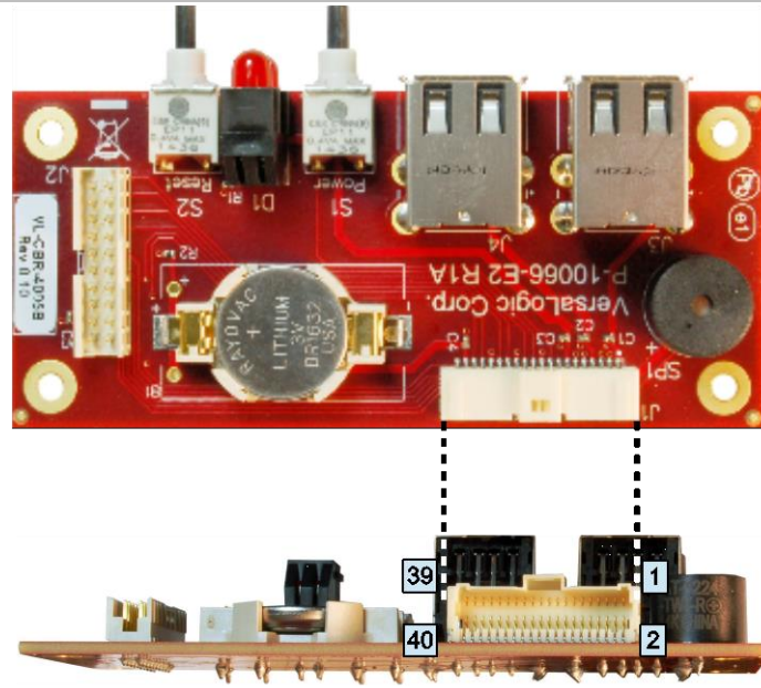
Figure 28. Location and Pin Orientation of the User I/O Connector
