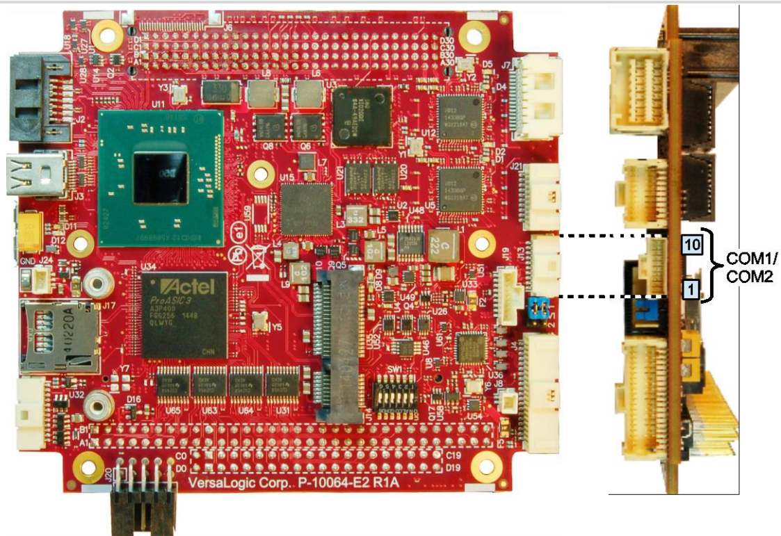
Figure 20. Location and Pin Orientation of Serial Port Connector
