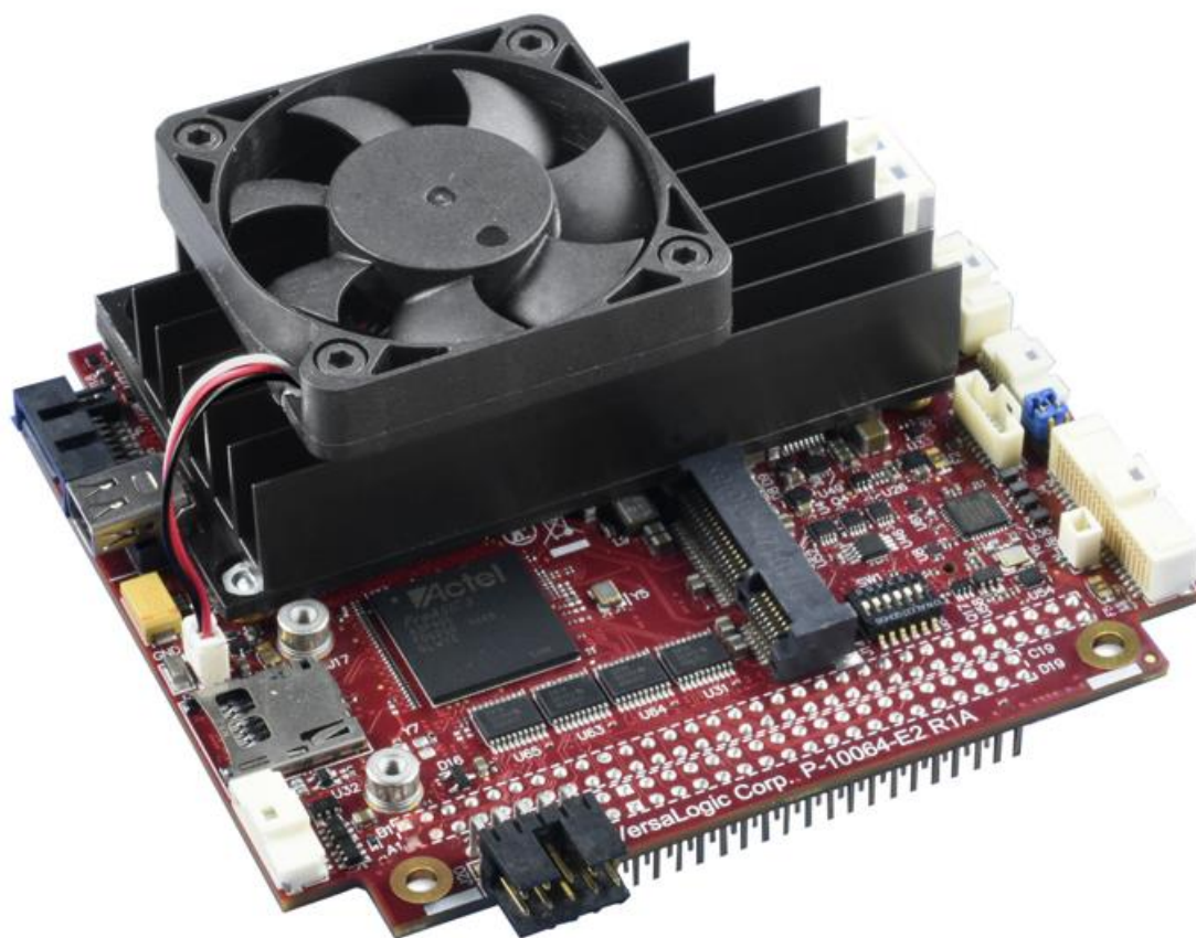
Figure 37. Installing the Heat Sink Fan
