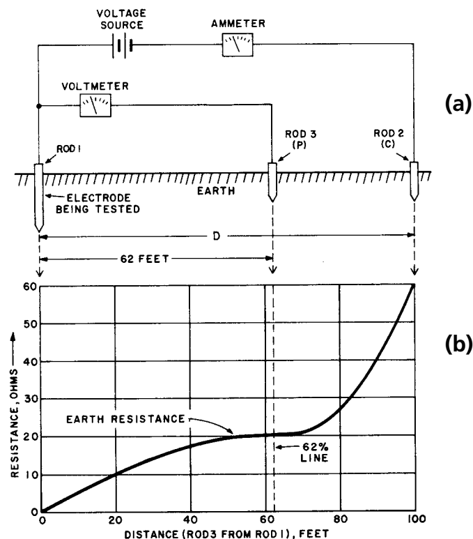
Fig. 10: Principle of an earth resistance test
