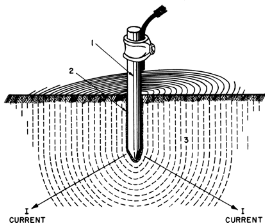
Fig. 9: Components of earth resistances in an earth electrode
