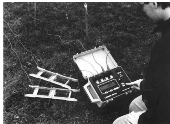
The Megger DET2/2 ground tester offers additional features for testing in a high-noise environment
