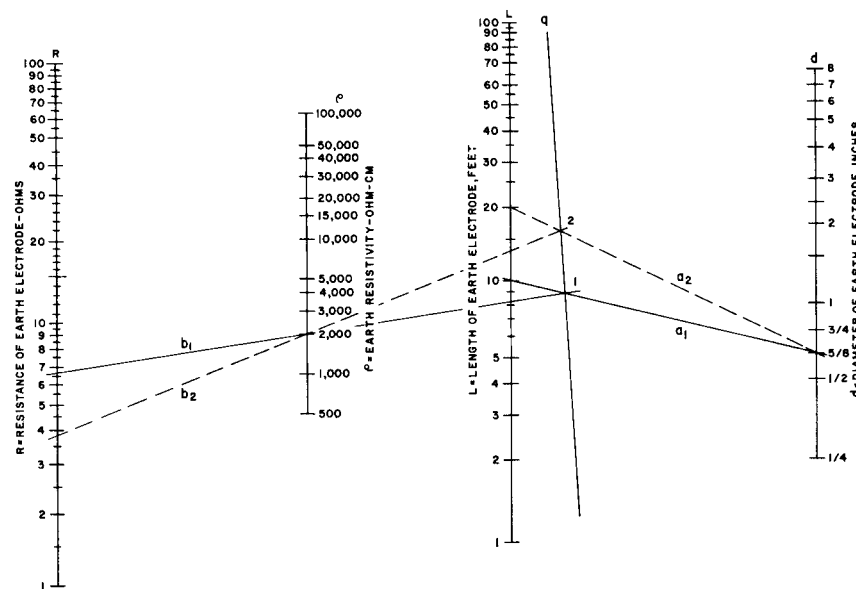
Fig. 21: Nomograph relating the basic factors affecting earth resistance.
