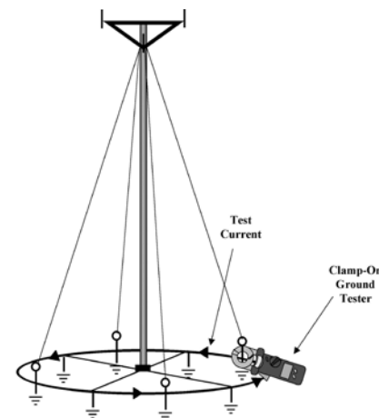
Fig 24: Cellular tower — example of a misused application
