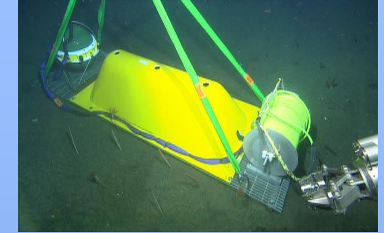
OBS Trawl resistant frame and cable spool
