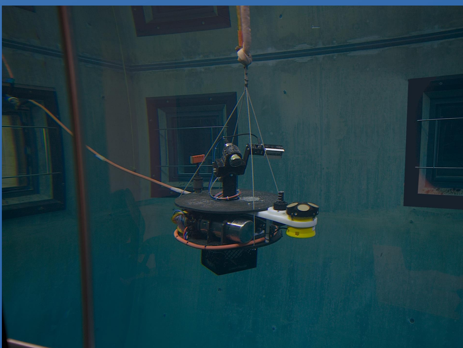
PhoBOS under test in tank
