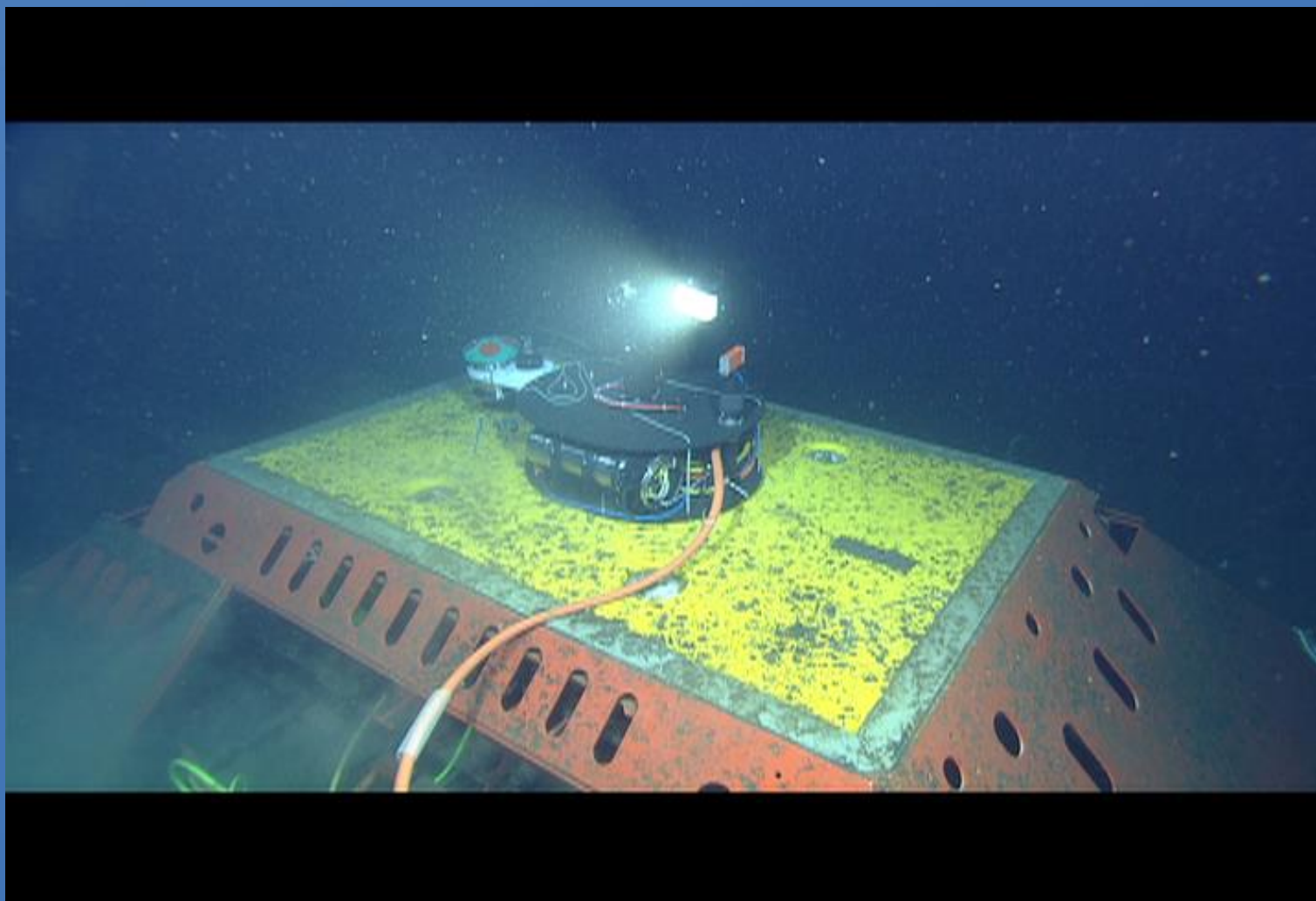
PhoBOS deploy and connected to MARS
