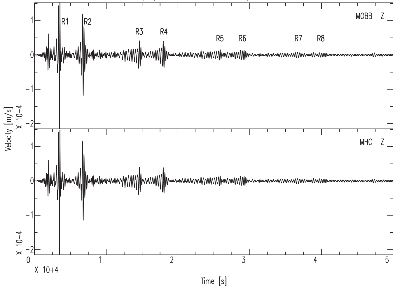
Sumatra 12/26/2004, Mw=9.3, Vertical Component, Filter 125–300s
