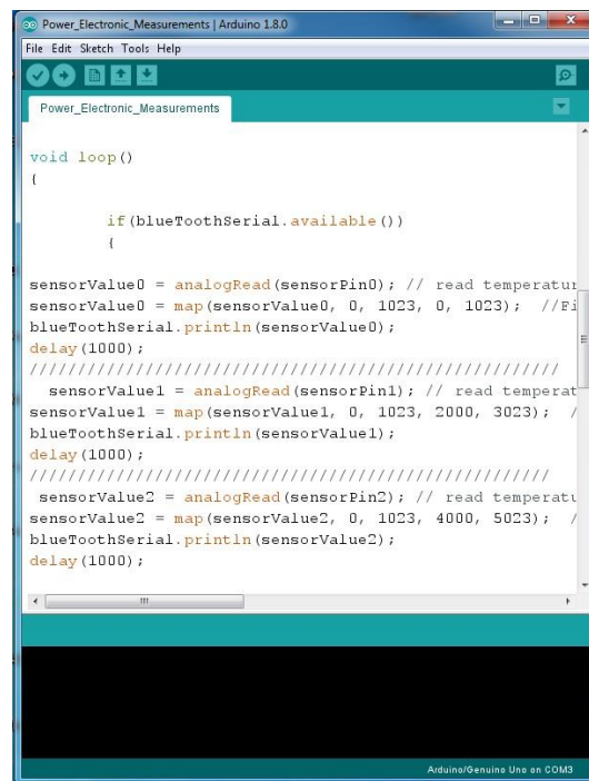
Figure 9. Main microcontroller program.
