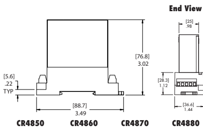
CR4870 3 Element, 4 Wire - 0 - 5 VDC Output
