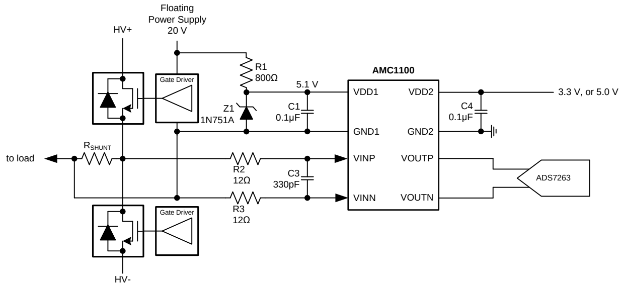
Figure 39. Zener Diode Based High-Side Supply
