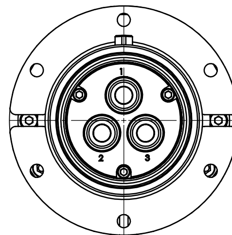
VIEW A-A SCALE 1:2
