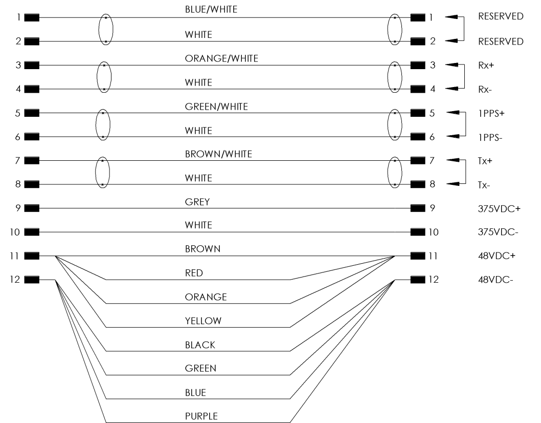
CIRCUIT DIAGRAM 1058159 (OPM-326-01-5) 1058161 (OPM-326-01-7)
