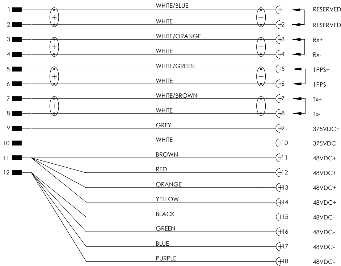
CIRCUIT DIAGRAM 1058160 (OPM-326-01-6) 1058162 (OPM-326-01-8)
