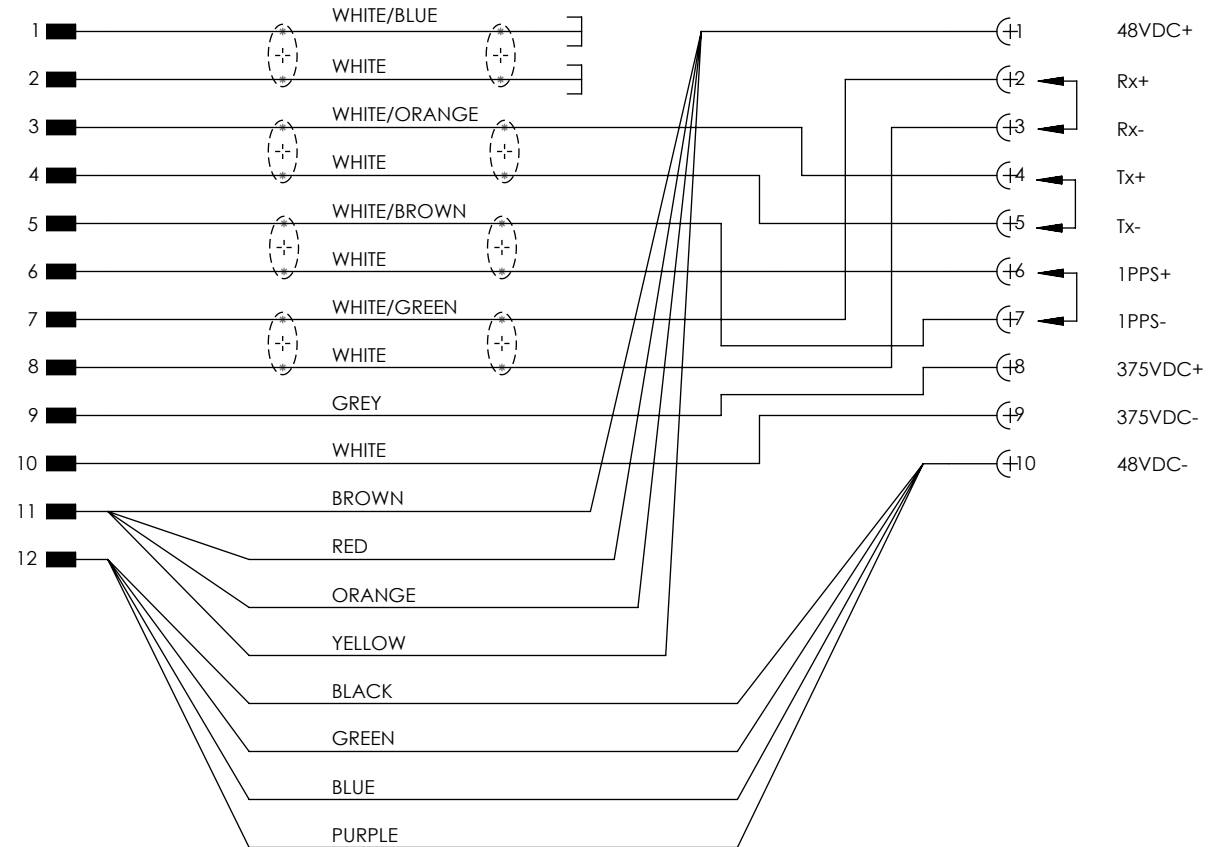
CIRCUIT DIAGRAM 1058660 (OPM-326-01-10)
