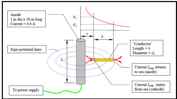
Figure 3. Stray current corrosion of a conductive object near the anode
