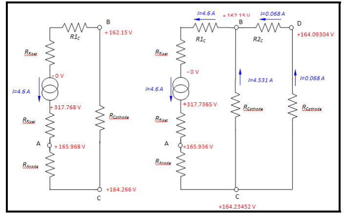
Figure 11. Equivalent circuit for parallel power feed of nodes 2 and 3 only (Left: One node; Right: Two nodes)
