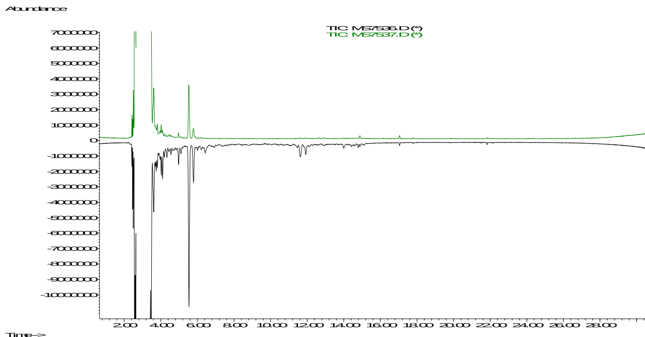
Figure 1. GC-MS chromatograms for the FC-77, Alcatel sample top and lab sample bottom.
