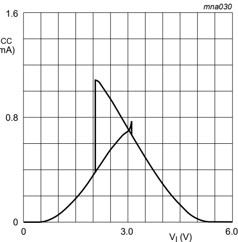
c. V_{CC} = 6.0\text{ V}
