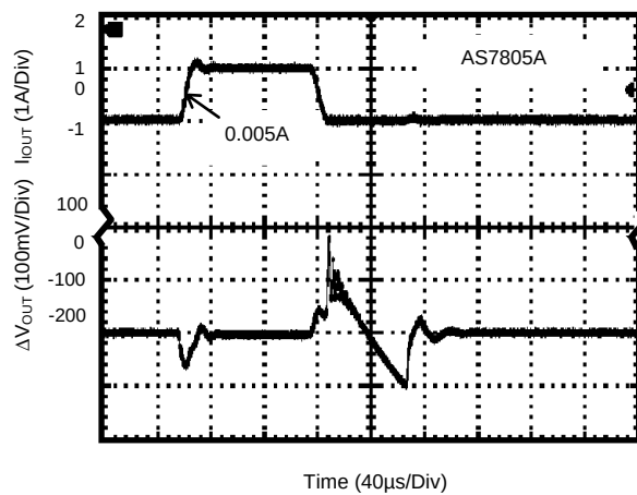
Load Transient (Conditions: V_{\text{IN}} = 10\text{V} , C_{\text{IN}} = 0.33\mu\text{F} , C_{\text{OUT}} = 0.1\mu\text{F} )
