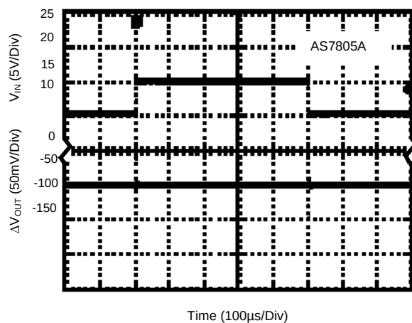
Line Transient (Conditions: I_{\text{OUT}} = 500\text{mA} , C_{\text{OUT}} = 0.1\mu\text{F} )
