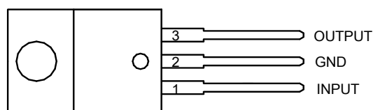
TO-220-3 (Option 2)
