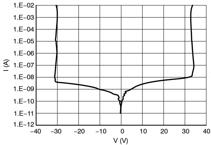
Figure 1. IV Characteristics
