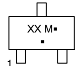
SC-70 CASE 419
