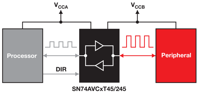
SN74AVCxT45/245 functional block diagram
