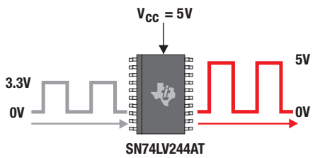
TTL up-translation
