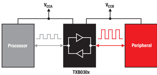
TXB030x functional block diagram
