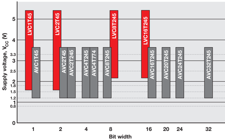
Direction-control translators
