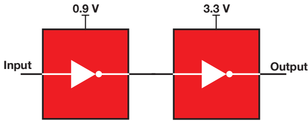
SN74AVC2T244/4T234 function block diagram
