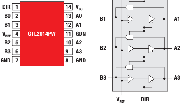
SN74GTL2014 functional block diagram
