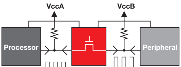
LSF010x functional block diagram
