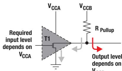
Translation with open-drain buffers
