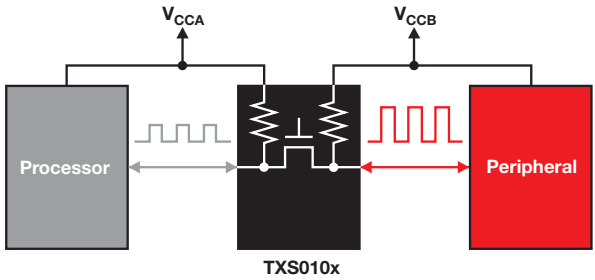
TXS010x functional block diagram
