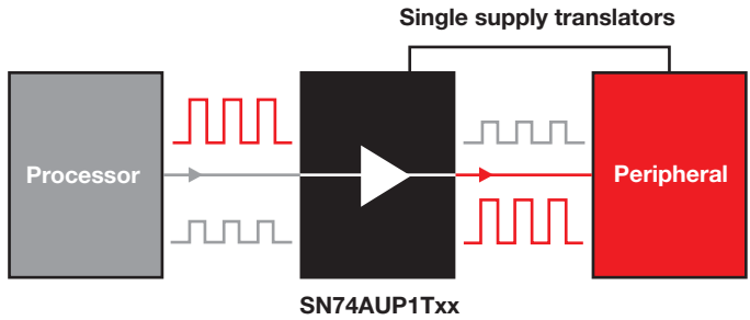
SN74AUP1Txx functional block diagram
