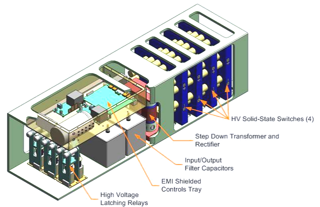
Figure 5. Simplified mechanical layout of the MVPC. Dimensions approximately 48" in length by 10.5" square.
