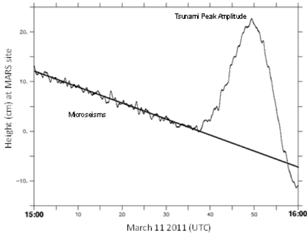
Figure 6. Nano-resolution pressure sensor at 40 Hz measures a 25 cm tsunami wave in Monterey Bay, California, which was a result of the Honshu, Japan earthquake on March 11, 2011.
