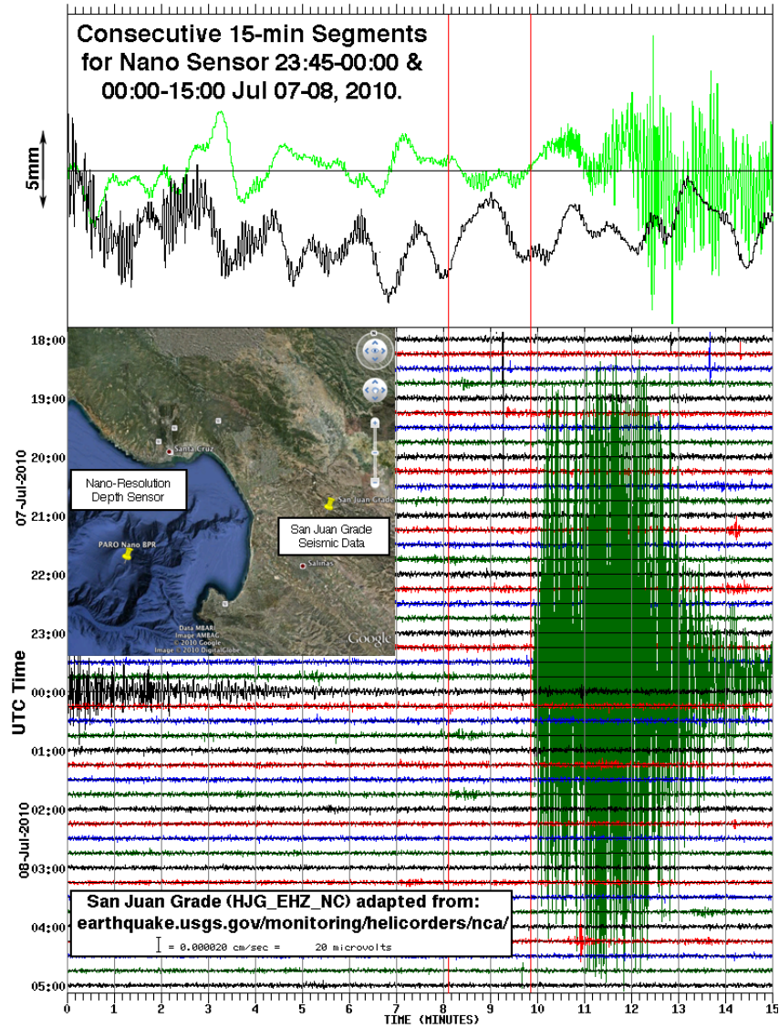
Figure 4. The upper panel shows consecutive 15-minute segments of the nano data (detrended) that correspond to the similarly colored traces in the USGS record from San Juan Grade in the lower panel. Inset is a locator map for the two locations which are separated by about 56 km. Vertical lines in red show the earthquake time and the arrival at the seismometer. The nano-resolution pressure sensor begins to respond a couple of minutes later and its earthquake signal has a similar duration to the land-based instrument.
