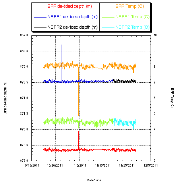
Figure 7. Pressure and temperature measurements of nano-resolution pressure sensor and standard BPR. The spike in the BPR de-tided depth time series (red) is due to transient temperature effects (orange) after a power cycle. In contrast, the spike in the nano-BPR de-tided depth time series (dark blue) is due to a known timing error and mismatch with a tide prediction model
