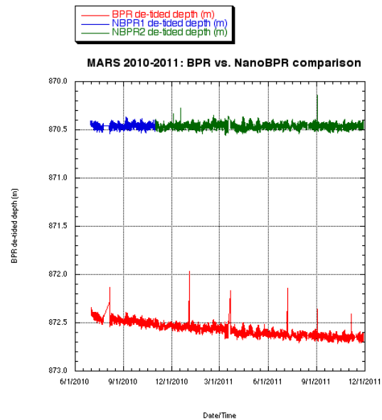
Figure 8. Pressure data (converted to depth) from nano-resolution pressure sensor and standard BPR over the entire 17 month deployment at MARS. The spikes in the BPR time series (red) are due to transient temperature effects after a power cycle. In contrast, the spikes in the nano-BPR time series are due to a known timing errors and mismatches with a tide prediction model
