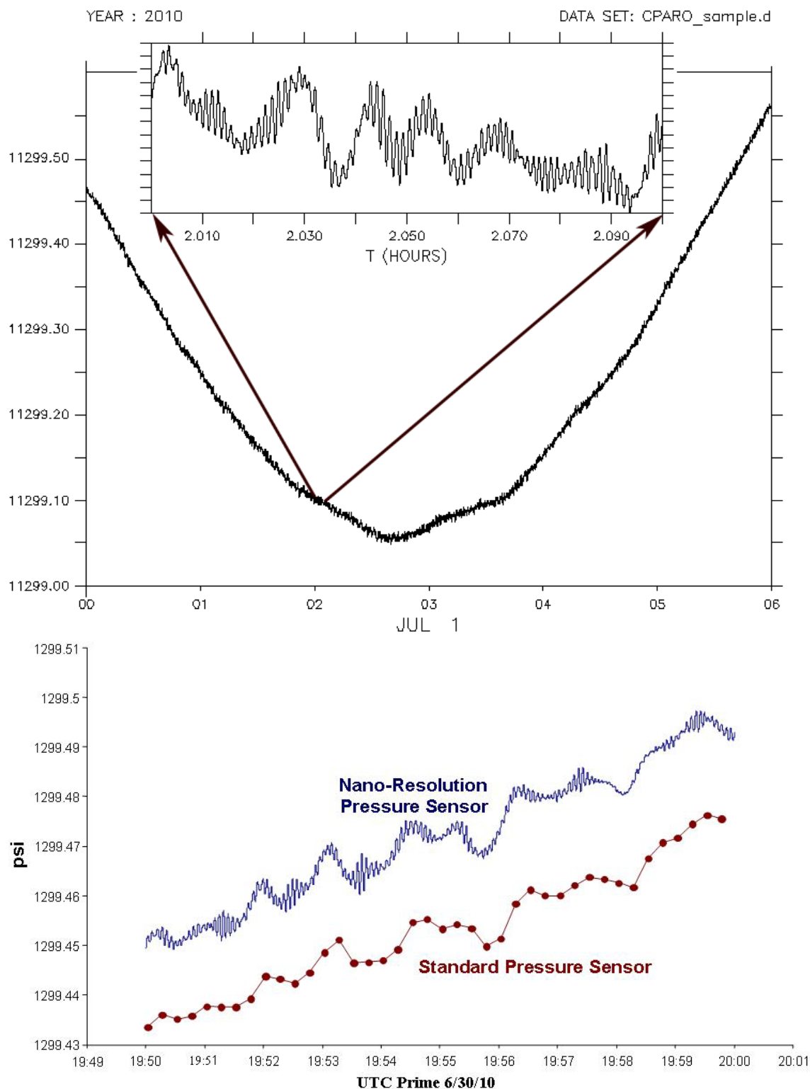
Figure 3. Nano-resolution pressure sensor data are shown (in blue on lower plot) hours after initial deployment. The overall pressure is rising from an incoming tide. Near 0.2 Hz, the data is dominated by microseismic acceleration of the seafloor (equivalent to 1 mm pressure variations). At longer periods, near 1 minute, pressure variations of a few millimeters water heights are from surface waves that are detected at the deployed depth of 900 m. The red data are from the co-located standard tsunami sensor at much lower sampling rate (15 seconds) and resolution (but still capable of resolving typical 1 mm waves at long periods). Note: the plots are arbitrarily offset to allow the reader to see differences in plotted data.
