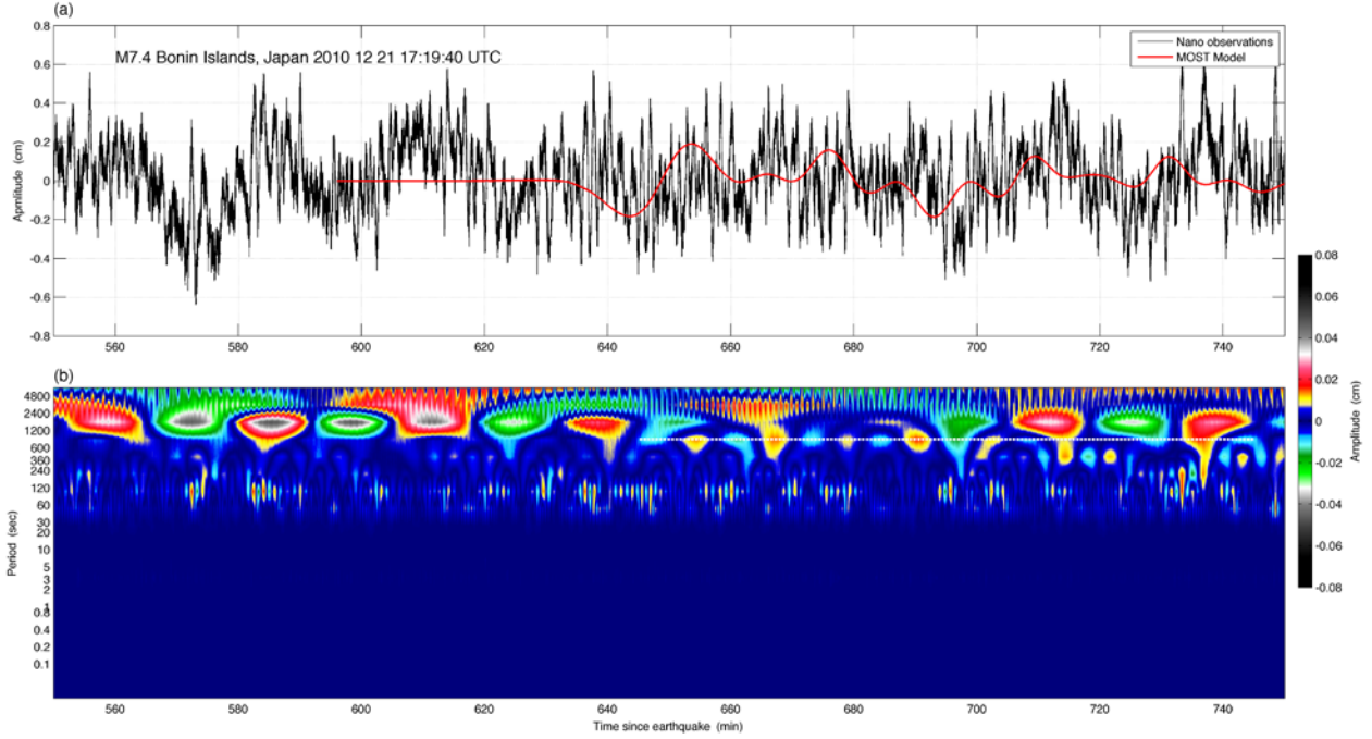
Figure 5. A micro tsunami generated by the M7.4 Bonin Island Earthquake on December 21, 2010 was recorded by the nano-resolution pressure sensor. (a) The black line is the nano-resolution observations with tides removed by a Butterworth filter with a cutoff period of 1 hour. The red line is the modeled tsunami amplitude time series. (b) Wavelet-derived amplitude spectrogram of the observations. The white dashed line indicates the existence of the tsunami signals.
