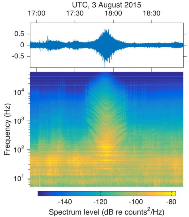
Fig. 7. Anthrophony: a typical boat transit detected by the hydrophone, represented as normalized waveform (top) and LTSA power spectral density (bottom).
