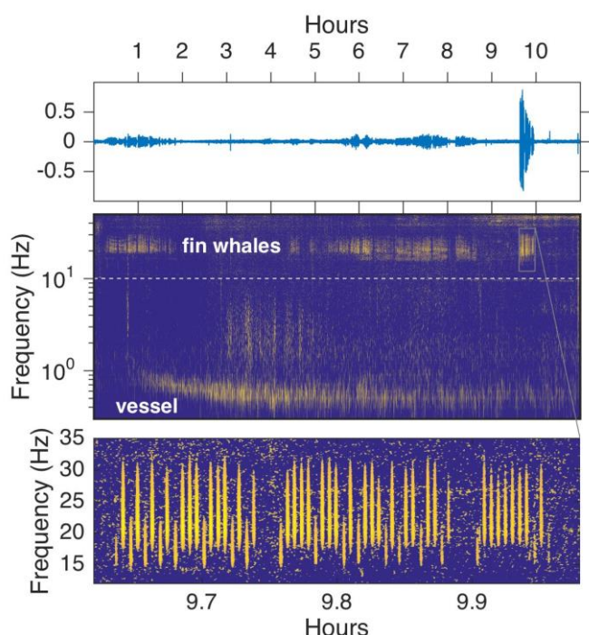
Fig. 8. Anthrophony: acoustic detection of distant shipping noise, specifically from the largest container vessel to dock in a US port, the CMA CGM Benjamin Franklin . The vessel transited offshore of the MARS hydrophone (Figure 1) during its first passage between the Ports of Los Angeles and Oakland. The start time of this recording is 30 December 2015 23:00 PST. Shown are waveform (top), the log of power spectral density (middle), and a zoom on the period of most active fin whale vocalization (bottom, domain delineated by the box in the middle panel). In the middle panel, the dashed line marks the low end of the range for the hydrophone's bandwidth specification.
