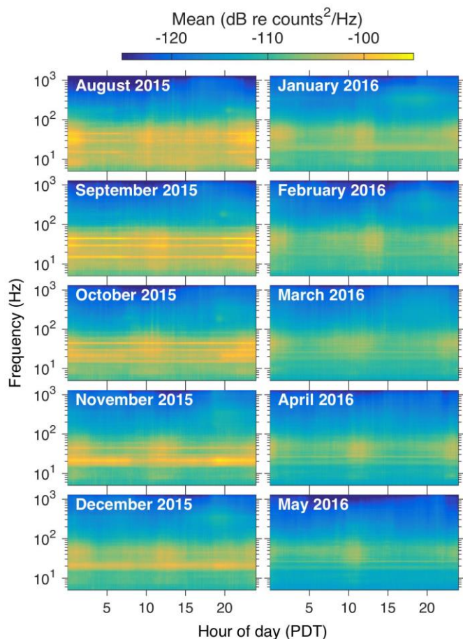
Fig. 2. Mean daily soundscape variations from low-frequency LTSA power spectral density (Table I) for the first 10 months of hydrophone data.
