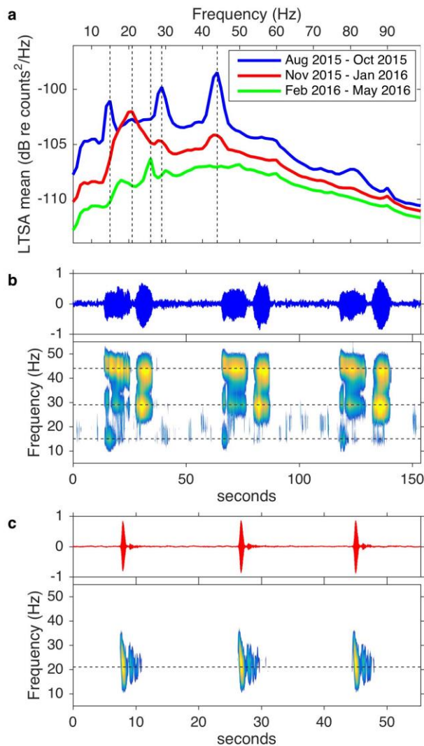
Fig. 3. Biophony: seasonal change in low-frequency vocalization energy. (a) Seasonal averaged LTSA spectra, computed from selected months of LTSA results (Figure 2). Months were grouped (legend) based on similarity of dominant patterns. (b) Example waveform and spectrogram plots of blue whale vocalizations (B calls and harmonics) causing the August – October peaks at 15, 29 and 44 Hz. (c) Example waveform and spectrogram plots of fin whale vocalizations causing the November – January peak at 21 Hz. MARS recordings in (b) and (c) were low-pass filtered with a 100 Hz cutoff and normalized for representing the waveform and spectrogram. Dashed lines in the spectrograms of (b) and (c) correspond with those defined in (a).
