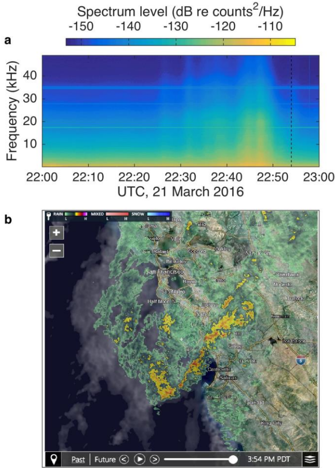
Fig. 6. Geophony: acoustic detection of a rain squall. (a) LTSA during one hour on 21 March 2016. (b) Weather radar image shows the squall line having passed over of the MARS location (image time indicated by the dashed line in (a)). The squall moved west to east.
