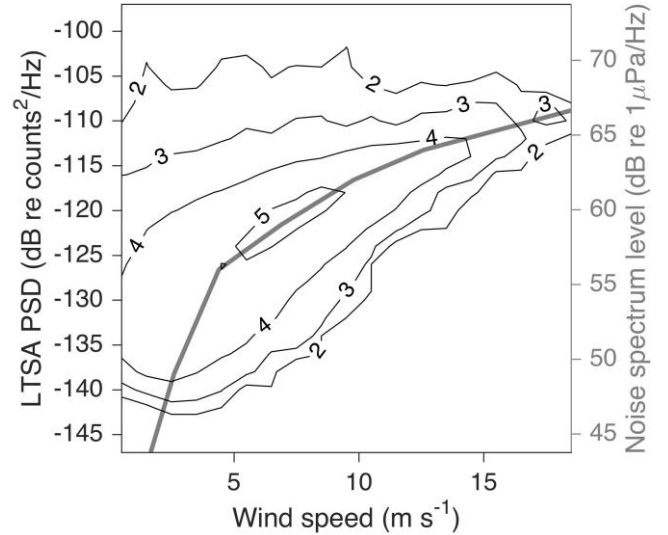
Fig. 5. Geophony: wind influenced sound. Relationship between wind speed measured at NDBC Station 46042 ( 36^{\circ}47'29'' N 122^{\circ}27'6'' W, 25 km WNW of MARS) and 2 kHz sound levels quantified by LTSA power spectral density of MARS hydrophone data. Contours are \log_{10} (number of observations). The thick gray line is the Wenz curve estimate at 2 kHz.
