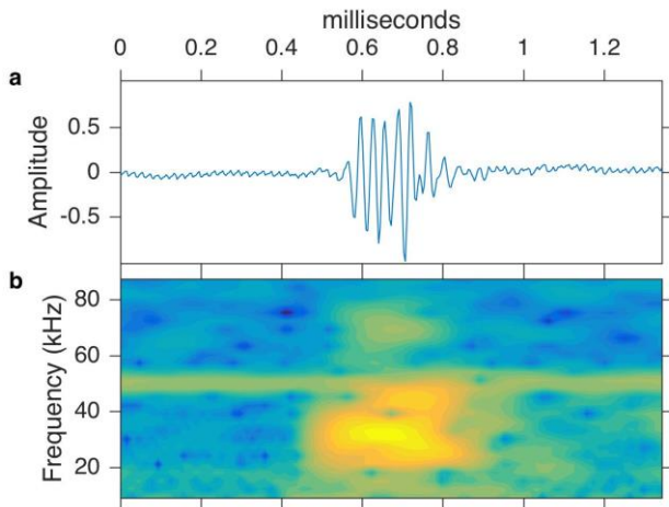
Fig. 4. Biophony: example of a beaked whale click detected on 28 October 2015, within a period of increased beaked whale click detections. (a) Waveform represented as normalized amplitude. (b) Spectrogram computed with nfft = 85 , overlap = 95 , and Hanning window; represented as relative spectral level. The continuous signal centered near 50 kHz is due to noise from the MARS power system.
