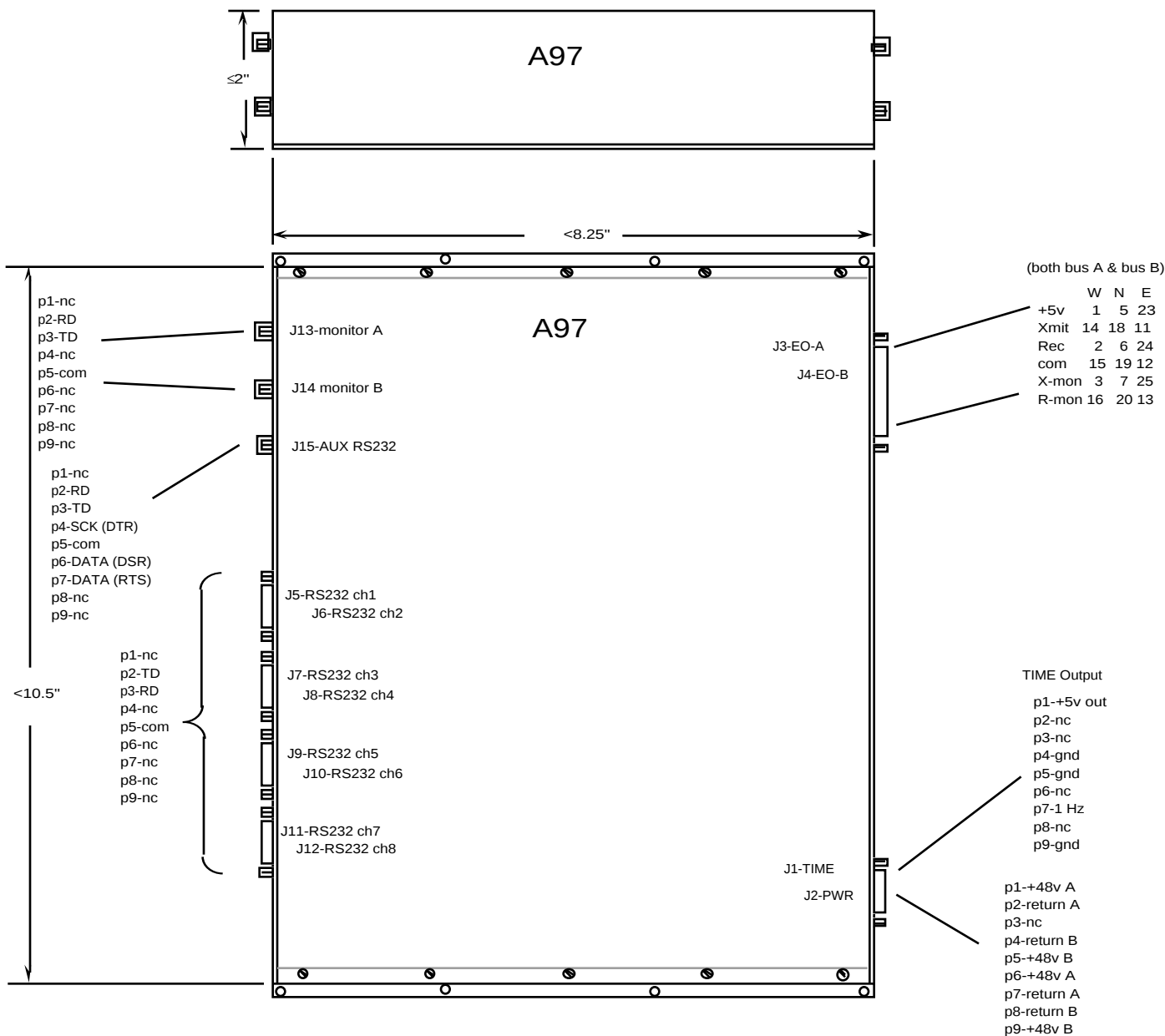
DB9 connector
