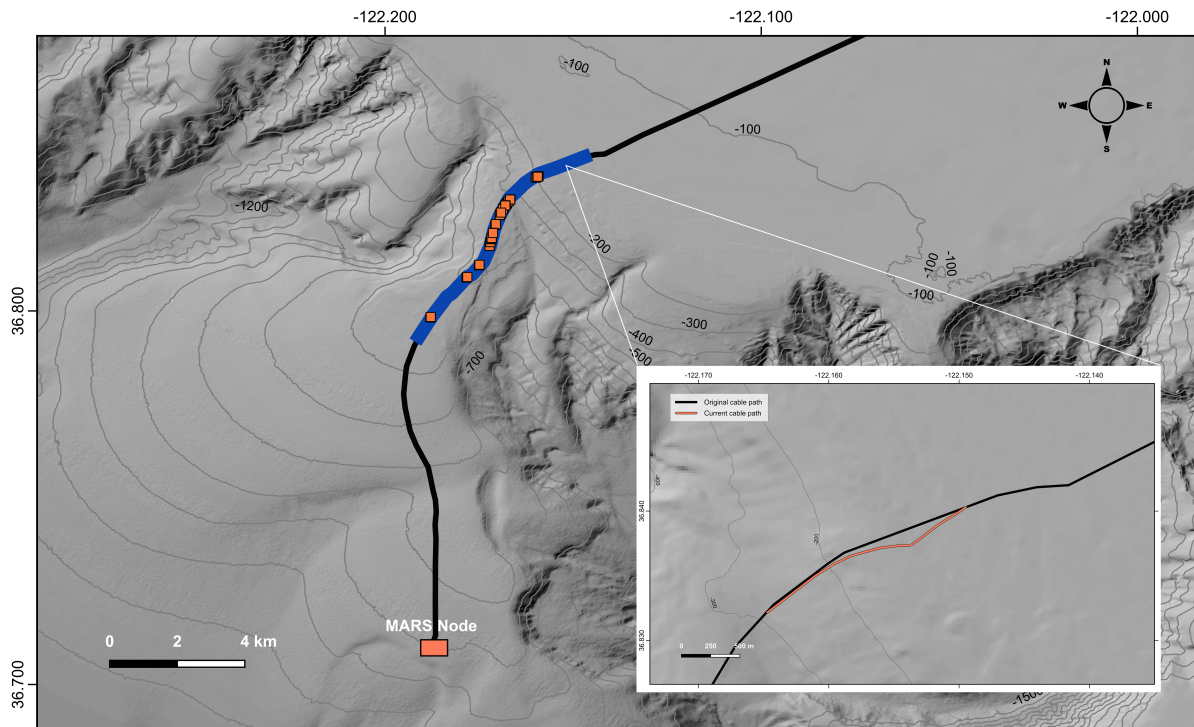
Figure 6. The MARS cable is buried along the entire route except for the area on the neck of Smooth Ridge, shown in blue. In 2020, the cable was 87% buried with 13% either exposed, partially buried or shallowly buried. Spans of the cable, as a result of minor topographic changes and rocks, are shown as orange markers within the area where the cable is exposed. Inset: A section of the cable has moved a maximum of 135 m to the SW, likely due to a trawling incident; the exact time frame for which this occurred is not known.
