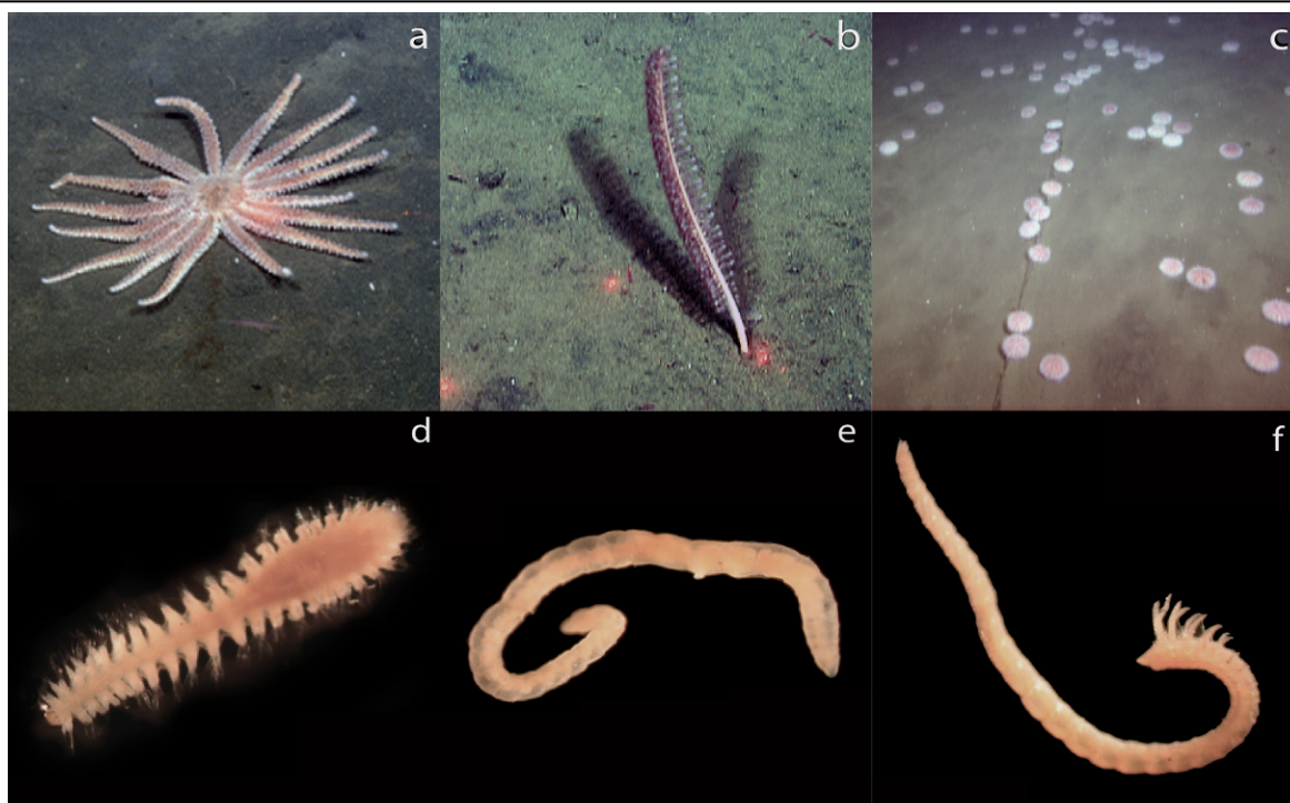
Figure 10. Some of the most abundant megafaunal and macrofaunal animals along the MARS cable route. A–C: Megafauna (ROV video transects): A. Rathbunaster californicus (sea star). B. Funiculina sp. (sea pen). C. Strongylocentrotus fragilis , (urchin). D–F: Macrofauna (sediment cores): D. Cossura sp. (polychaete worm). E. Oligochaeta . F. Prionospio sp. (polychaete worm).
