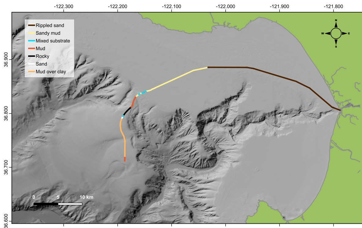
Figure 5. Substrate composition along the MARS route.
