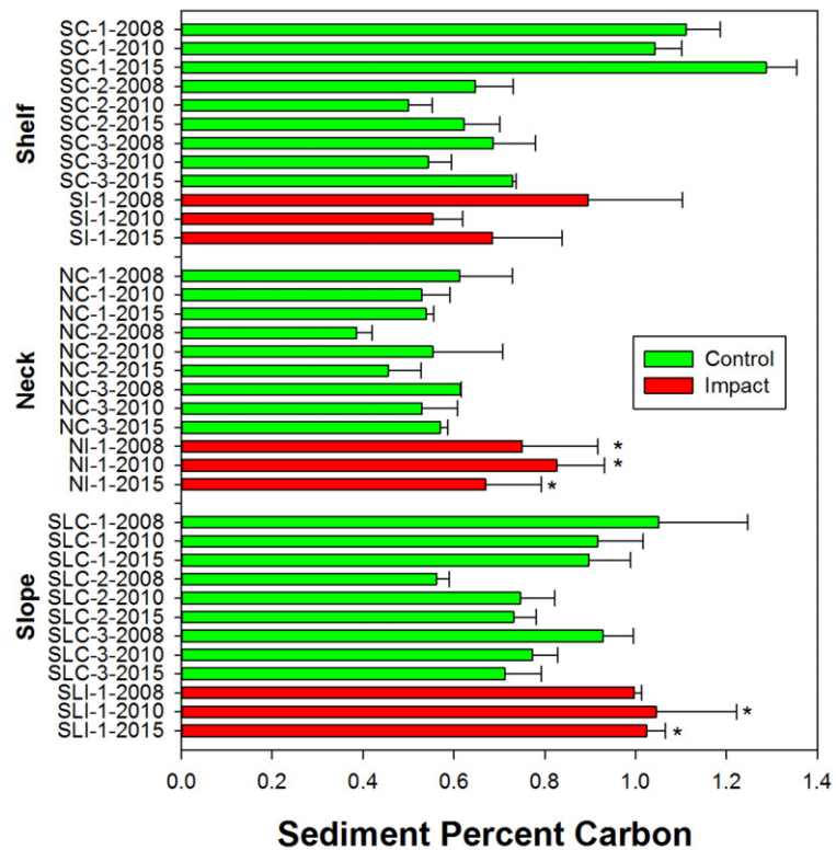
Figure 8. Mean percent organic carbon in surficial sediments for control and cable sites at the three cable depth regions (+/- SD). Comparisons of control vs. cable (impact) sites was nonsignificant for the Shelf region ( p = 0.35 ). Differences were significant for Slope ( p = 0.002 ) and Neck depths ( p = 0.001 ). * = significant difference between control and impact areas for the sampling period.
